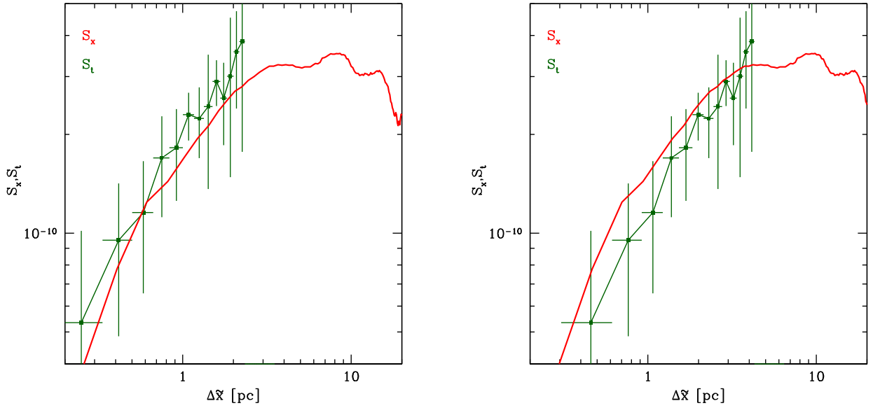
Figure 4. Same as in Fig. 2 for \eta = 0.3 (left) and \eta = 1 (right). In terms of elapsed time since the outburst the figures correspond to \sim 250 and \sim 75 yr, respectively. Clearly the agreement between the structure functions is much poorer than for \eta = 0.7 .
