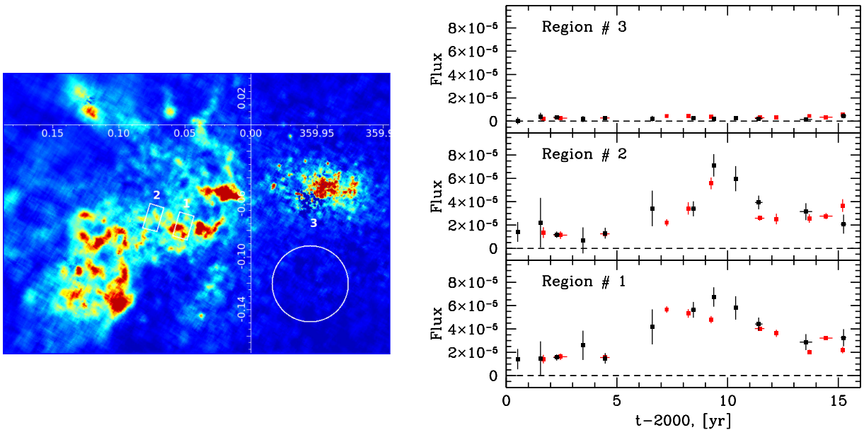
Figure 5. Light curves of reflected emission for selected regions. Left: three regions used for the analysis, superposed on to the Chandra map. Regions 1 and 2 are located within the molecular complex bright in reflected emission. Region 3 is a test region where reflected emission is faint. Right: light curves for regions 1, 2 and 3 (from bottom to top). Red and black points correspond to XMM-Newton and Chandra observations, respectively. The duration of the peaks sets an upper limit on the duration of the outburst. Even for an extremely short outburst the finite spatial extent of each cloud along the line of sight broadens the peak. For instance, for a cloud with size of 1 pc, the minimum duration of the observed outburst, given \frac{\partial z}{\partial t} \sim 0.75c is 4.3 yr.
