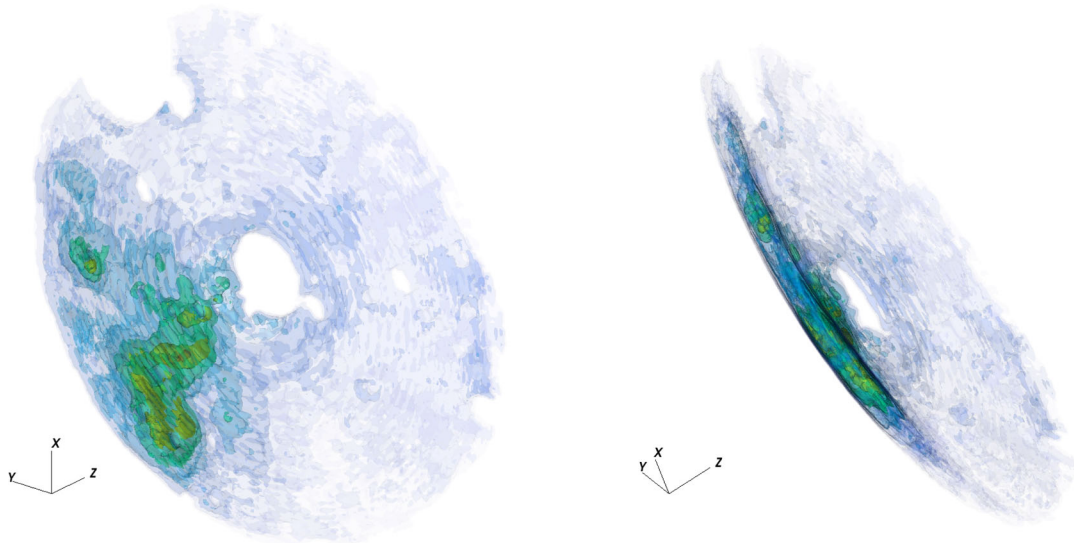
Figure 7. 3D distribution of gas near the Galactic Center based on our fiducial model of a short flare 110 yr ago. The locus of the illuminated points at any given time is a paraboloid [see equation (5)]. The surface brightness at location (l, b) observed by XMM-Newton at time t is recalculated to the gas density (scaled by a fiducial value of total fluence) and placed into a cell with coordinates (l, b, z) . The radius of the studied area is \sim 35 pc. The thickness of the paraboloid along the line of sight covered during \sim 15 yr of XMM-Newton observations is \sim 0.75 \times c \times 15 \text{ yr} \approx 3.4 pc. Left-hand and right-hand panels show different orientations of the same data cube. The ‘holes’ correspond to excised regions contaminated by bright compact sources. VisIt software package was used to generate this figure (Childs et al. 2012).
