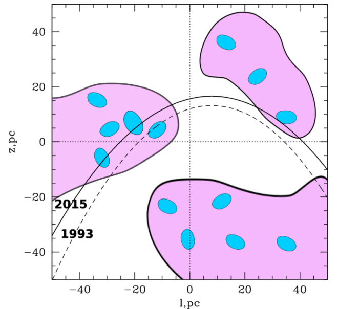
Figure 3. Sketch of a short outburst scenario for the outburst that happened \sim 110 yr ago, assuming that the primary source is at (0,0) . This is a view on the Galactic Center region from the Galactic pole, with the galactic longitude l along the horizontal axis, and the line-of-sight distance z along the vertical axis. The dashed and solid lines correspond to the position of the ‘light-front’ in 1993 and 2015, respectively. The distance along the line of sight between the illuminated regions is given by \sim \frac{\partial z}{\partial t}(t_2 - t_1) , where t_2 - t_1 \sim 22 yr (see text). For regions close to primary source in projection, the value \frac{\partial z}{\partial t} \sim 0.5c . This value increases with projected distance from the primary source.
