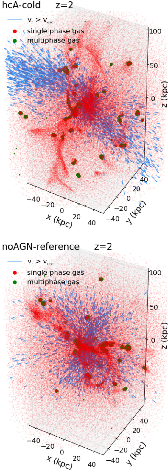
Figure 12. Geometry of the outflowing gas in the hcA-cold model and in the reference simulation with no AGNs, at z = 2 . Single-phase gas is shown by red points, multiphase gas by green dots, and is mostly embedded within the innermost regions of the forming galaxy. Light blue arrows pinpoint gas that is outflowing with a radial velocity larger than the escape velocity of the halo (see Table 6 for details).
