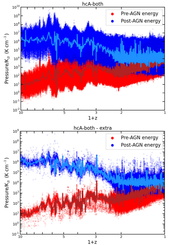
Figure 7. Pressure of multiphase gas particles before and soon after the feedback energy injection, as a function of redshift, for the simulation hcA-both. Solid curves show the median evolution. Top panel: evolution of gas particles for which all the feedback energy supplied to the cold gas is used for the evaporation of the cold gas mass. Bottom panel: evolution of gas particles for which a fraction of the energy initially allocated to the cold phase is provided to the hot phase, as an additional contribution that ensures that no feedback energy is lost.
