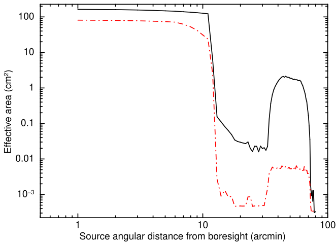
Figure 3. The effective area of the XRT as a function of off-axis angle, derived from ray-tracing simulations. The focused field of view is 12\frac{2}{3} in radius. The solid black curve shows the total effective area for a point source, integrated over the entire CCD, as a function of off-axis angle. The broken red line shows the peak effective area, which occurs in a CCD area equivalent to the half-energy width of the PSF ( 18'' diameter). The two curves are more disparate for sources outside the nominal field of view, because the X-rays for these are spread out over a much larger area of the CCD in large rings, whereas for on-axis sources, the counts are focused into the spot-like point-spread function.
