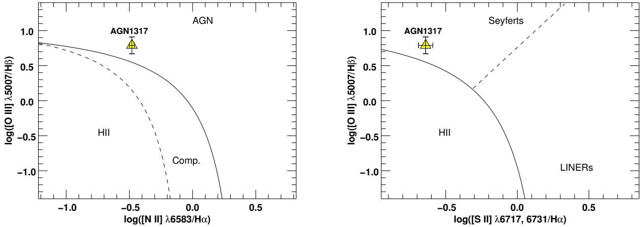
Fig. 8. Baldwin et al. (1981; BPT) diagrams. Left panel: [N\ II]/H\alpha vs. [O\ III]/H\beta BPT diagram showing the location of AGN1317 (yellow triangle). We adopted the classification of the galaxies in H II-region-like, composite AGN-H II types, and AGN according to Kewley et al. (2006). The Kewley et al. (2001) extreme starburst line and the Kauffmann et al. (2003) pure star formation line are shown as the solid and dashed lines, respectively. Right panel: same as the left panel for the [S\ II]/H\alpha vs. [O\ III]/H\beta BPT diagram. We adopted the classification of the galaxies in H II-region-like, Seyferts, and LINERs according to Kewley et al. (2006). The Kewley et al. (2001) extreme starburst line and the Kewley et al. (2006) Seyfert-LINER line are shown as the solid and dashed lines, respectively.
