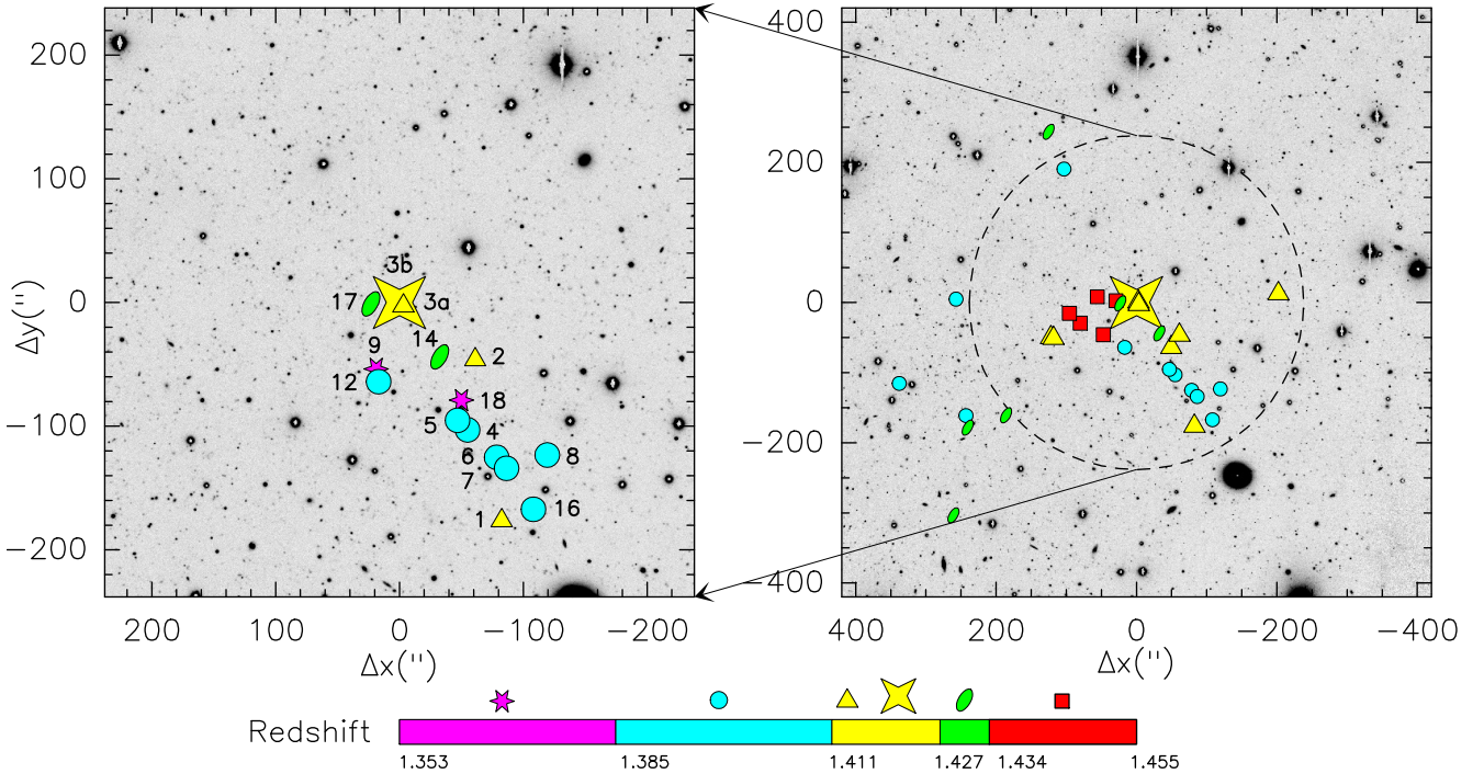
Fig. 4. Left panel: galaxies we spectroscopically detected in the field of the overdensity around radio galaxy 7C 1756+6520 plotted in the B-band image (NOAO). They comprise protocluster members, possible protocluster members, and non protocluster members (see Table A.1). ID numbers, corresponding to the slit, are provided for each source (see Table A.1). The five colors and symbols indicate different redshift ranges: magenta stars z < 1.385 , light blue circles 1.385 \leq z \leq 1.411 , yellow triangles 1.411 < z < 1.427 , green ellipses 1.427 \leq z \leq 1.434 , and red squares (in the right panel) z > 1.434 . The central radio galaxy 7C 1756+6520 is the large yellow star in the center. North is up and east to the left. The FoV is about 480'' \times 480'' , centered on the central radio galaxy. 1'' corresponds to \sim 8.4 kpc. Right panel: all protocluster and possible protocluster members with spectroscopically confirmed redshift from this work, G 10, and M 12. Symbols and colors are the same as in the left panel. The FoV is 840'' \times 840'' . The dashed circles indicate a distance of 2 Mpc from the central radio galaxy.
