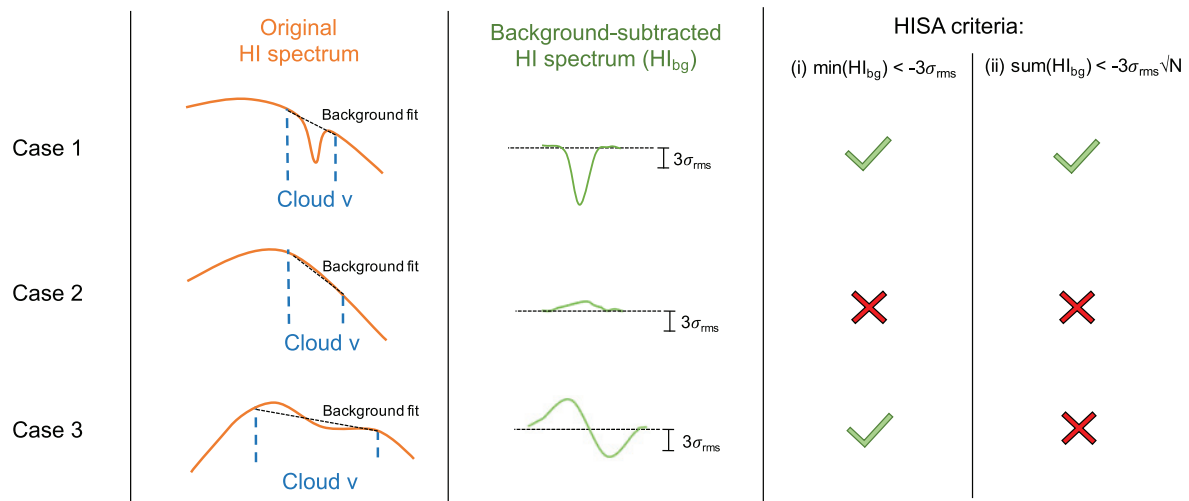
Figure 7. Three sketch examples of the automated HiSA method, showing the original H I spectrum on the first column (in orange), with the cloud’s velocity ranges denoted in blue, and the linear background fit done to the H I spectrum in black dotted line. The second column shows the cloud’s background-subtracted H I spectra (in green), with the dotted dashed line representing the 0-emission level, and the vertical bar representing 3\sigma_{\text{rms}} of the H I emission. The two last columns show the criteria that we use to infer whether there is HiSA in that particular sightline. Case 1 represents a line of sight with strong HiSA, but the other two cases are not considered to have HiSA. Case 3 shows an example of a false positive arising from criterion (i) alone, but which is mitigated by introducing criterion (ii).
