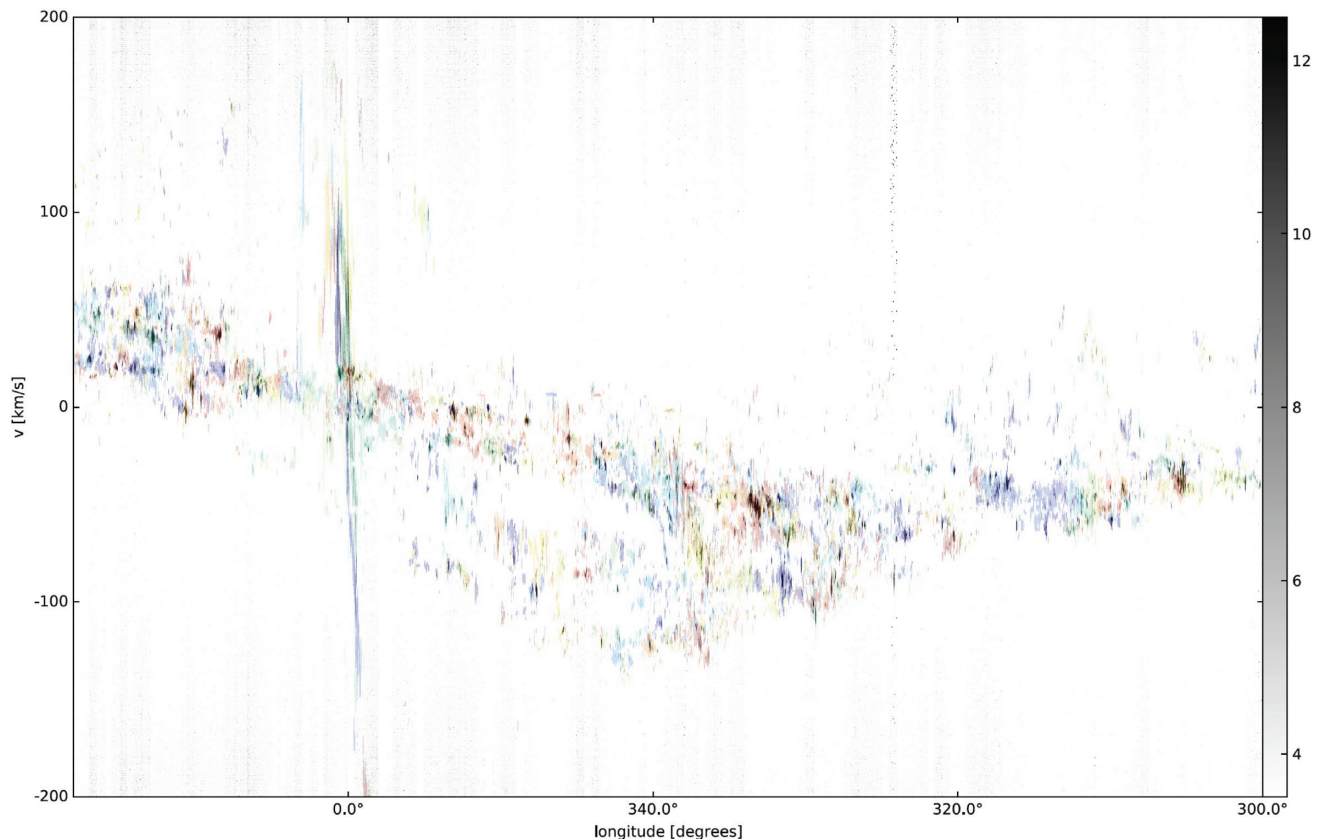
Figure 1. Longitude–velocity ( \ell v ) map of the ^{13}\text{CO} peak intensity (in grey-scale) for the SEDIGISM coverage analysed in this paper. The peak intensity map was built after masking out voxels of the ^{13}\text{CO} datacube with intensities < 2.5\sigma_{\text{rms}} (estimated locally for each line of sight). The clouds extracted with SCIMES are overlaid as colours, where each cloud has a different (random) colour.
