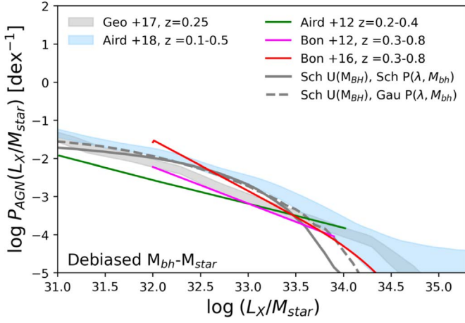
Figure 9. Left panel: specific accretion rate distribution P_{\text{AGN}}(\lambda, M_{\text{star}}) given by the convolution of the input BH mass-dependent Eddington ratio distribution P(\lambda, M_{\text{BH}}) and AGN duty cycle. The prediction from mock AGNs with a Schechter (solid line) and Gaussian (dashed line) P(\lambda, M_{\text{BH}}) and an M_{\text{star}}-M_{\text{BH}} relation as defined in Shankar et al. (2016) are compared with data as in Figure 4. Right panel: large-scale bias vs. X-ray (2–10 keV) luminosity (in units of \text{erg s}^{-1} ) for mock AGNs when using an input Eddington ratio distribution that is independent of (dependent) the BH mass for a decreasing (Schulze & Wisotzki 2010) and constant ( U = 0.2 ; Goulding et al. 2010) duty cycle as a function of BH mass, compared with bias estimates from previous studies at similar redshifts.
