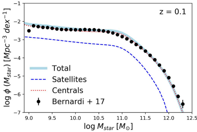
Figure 1. Left panel: stellar mass function at z = 0.1 for central and satellite mock galaxies, compared with measurements using SDSS DR7 galaxies. Right panel: BH mass–stellar mass relation, as put forward by Shankar et al. (2016, debiased) and derived for local galaxy samples with dynamically measured BH masses from Savorgnan & Graham (2016, raw). The M_{\text{BH}}-M_{\text{star}} relations as derived for early- and late-type galaxies by Sahu et al. (2019) and AGNs by Reines & Volonteri (2015) are shown for comparison.
