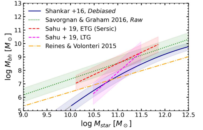
Figure 1. Left panel: stellar mass function at z = 0.1 for central and satellite mock galaxies, compared with measurements using SDSS DR7 galaxies. Right panel: BH mass–stellar mass relation, as put forward by Shankar et al. (2016, debiased) and derived for local galaxy samples with dynamically measured BH masses from Savorgnan & Graham (2016, raw). The M_{\text{BH}}-M_{\text{star}} relations as derived for early- and late-type galaxies by Sahu et al. (2019) and AGNs by Reines & Volonteri (2015) are shown for comparison.
