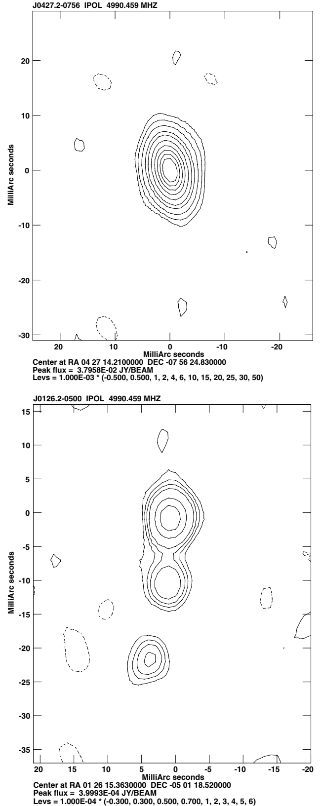
Fig. 1. Total-intensity images of the point-like source J0427.2–0756, the core-jet source J0126.2–0500. The convolution beams are 7.6 \times 4.3 mas at 14.8^\circ , 6 \times 6 mas, respectively.
