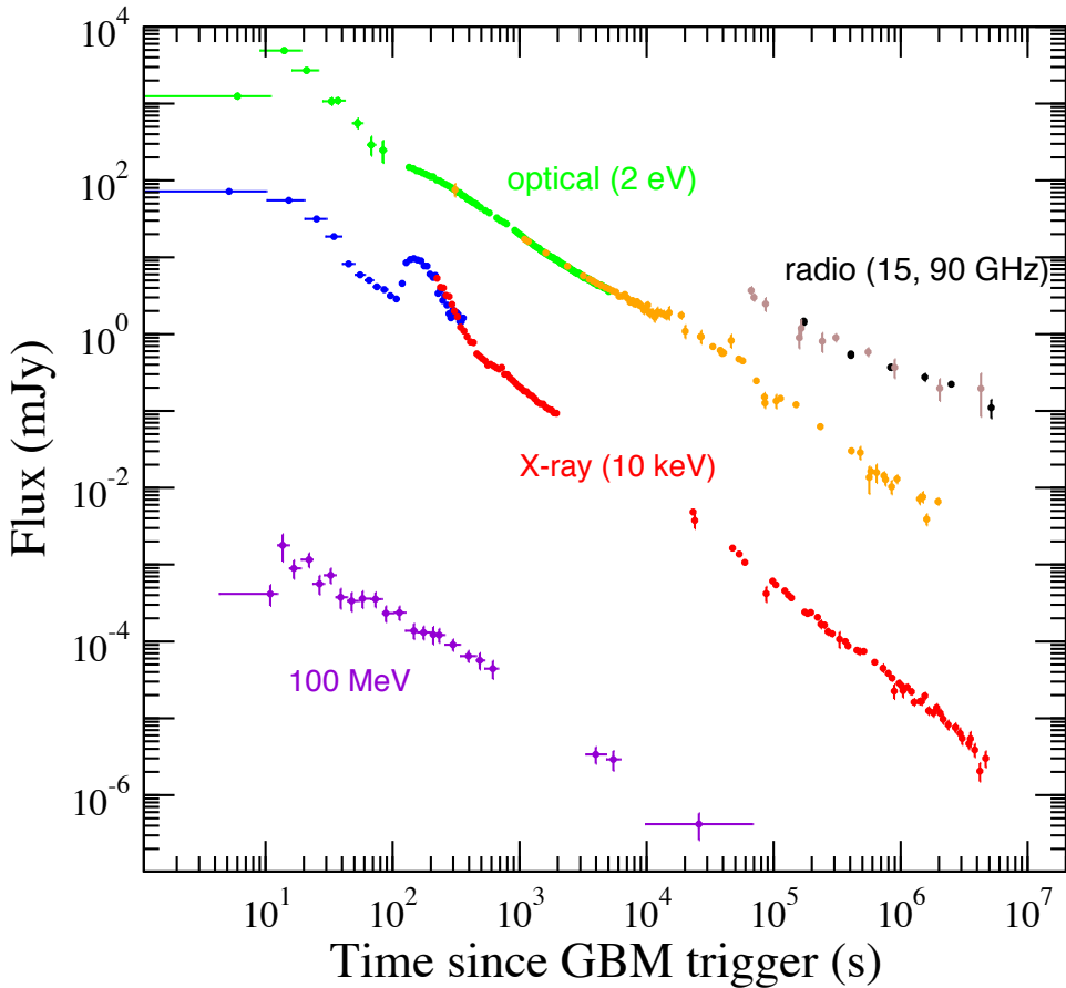
Figure 4: Example of a GRB afterglow in different spectral ranges. The data reported are for GRB 130427A afterglow (Panaiteescu et al. 2013). (Figure courtesy of Alin Panaiteescu).
