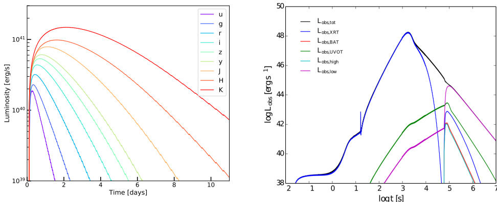
Figure 6: Left : KN lightcurve in different photometric filters (optical and NIR) from a single component model characterized by M_{\text{ej}} = 0.01 M_{\odot} , v_{\text{ej}} = 0.1c and k = 10 \text{ cm}^2/\text{g} . Lightcurves obtained with the code in https://github.com/mcoughlin/gwemlightcurves . Right : SDPT lightcurve from the fiducial model in Siegel & Ciolfi (2016b) characterized by M_{\text{ej}} = 5 \times 10^{-3} M_{\odot} and B = 10^{16} \text{ G} . In this case the NS does not collapse. Black curve represents the bolometric luminosity, the dark blue curve is the lightcurve in the energy range of Swift -XRT (0.3-10 keV), the red curve in Swift -BAT range (15-150 keV), the green curve in Swift -UVOT range (170-650 nm). Light blue and purple curves represent lightcurves above BAT range and below UVOT range, respectively. Figure adapted from Siegel & Ciolfi (2016b).
