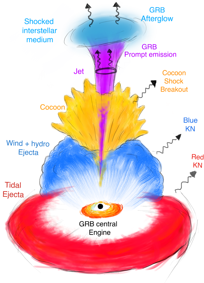
Figure 2: Artistic representation of the scenario following a NS-NS/NS-BH merger, when an accreting BH is formed. The red component denotes the tidal ejecta, the blue component the hydrodynamic and wind ejecta, the purple component the jet and the yellow component the matter of the ejecta heated by the jet (cocoon). The different components are not represented in scale.
