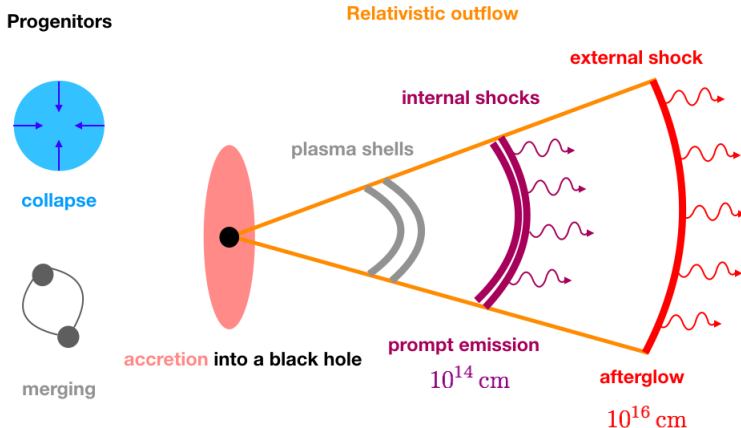
Figure 5: Pictorial representation of the basic model of the GRB: the core-collapse of a massive star or the coalescence of a NS-NS (or NS-BH) leads to the formation of an accreting BH, which launches an ultra-relativistic outflow in a form of a jet. Internal dissipation of the jet’s kinetic energy through shocks produces the prompt emission in the keV-MeV range. The forward shock of the jet with ambient medium forms the afterglow radiation observed in the X-ray, optical and radio bands.
