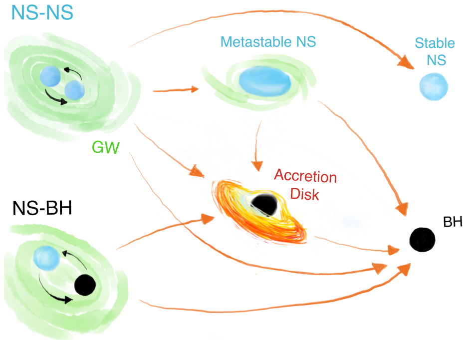
Figure 1: Different scenarios for a NS-NS and a NS-BH merger and the merger remnant. The EM radiation is expected when an accretion disk and unbound mass are left outside the merger remnant.
