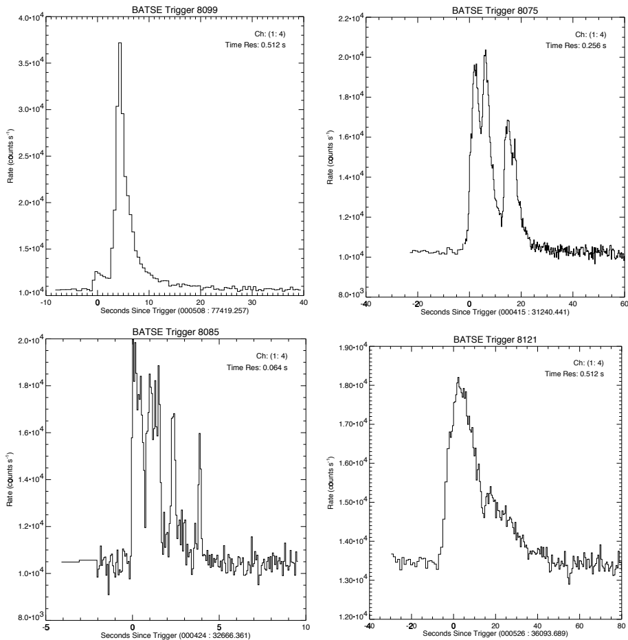
Figure 3: Examples of GRB prompt emission lightcurves ( E > 20 keV) from the online BATSE catalog: https://gammaray.nsstc.nasa.gov/batse/grb/lightcurve/
