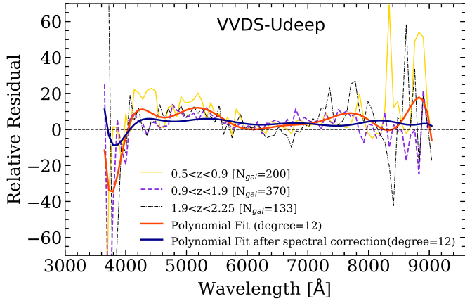
Fig. 1. Median spectral residual estimated from the fit of our selection of galaxies with SPARTAN in the VVDS Ultra-Deep survey. We show the relative residual in three redshift bins: 0.5 < z < 0.9 (yellow line), 0.9 < z < 1.9 (purple dashed line), and 1.9 < z < 2.25 (black dot-dashed line). We indicate the number of fits used in the estimation of the residual for each redshift bin. We also show the polynomial fit of the average residual before (orange thick line) and after (blue thick line) spectral correction. The fit is performed on the average of all the redshift bins and enters in the correction of the spectroscopy.
