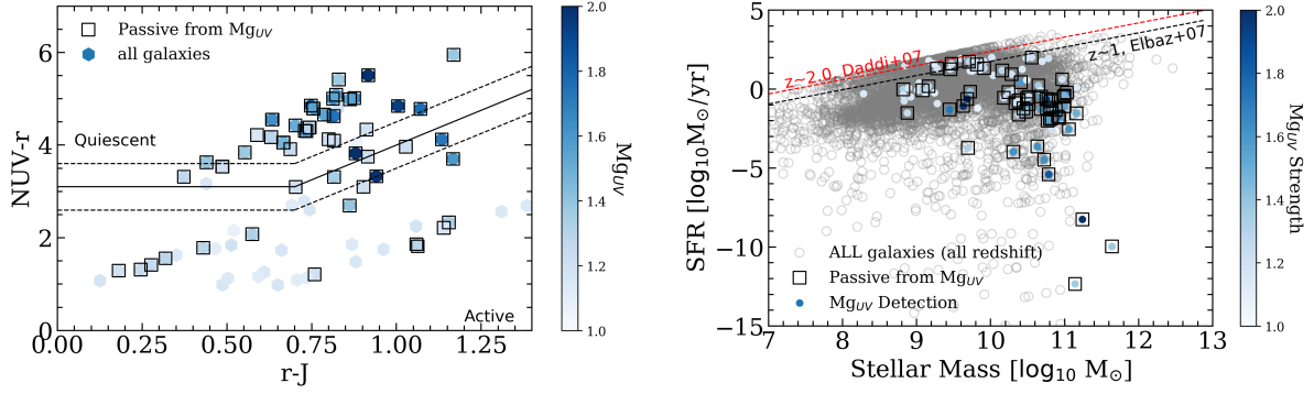
Fig. 9. Left: NUVrJ color-color diagram for all our selected galaxies. The value of M_{\text{UV}} galaxies in our sample is color-coded. We identify the galaxies selected as passive using the M_{\text{UV}} index only by empty black squares. The passive region (black solid and dashed line) is taken from Davidzon et al. (2017). Right: position of our galaxies in the M-SFR diagram. We show in gray all the galaxies from VVDS deep and ultra deep sample (at all redshift) for comparison. We also show the main sequence fit at z \sim 1 and 2 from Elbaz et al. (2007) and Daddi et al. (2007), respectively. Our selected galaxies are shown in color representing the M_{\text{UV}} strength.
