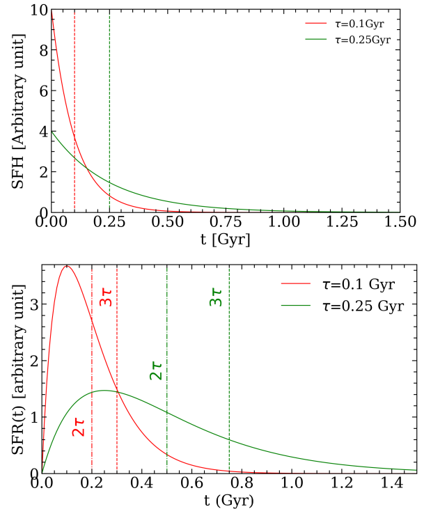
Fig. 7. Comparison of the Age_{passive} definition between exponentially declining SFH (top panel) and exponentially delayed SFH (bottom panel). In each case we show the position of different timescales with dashed vertical lines.
