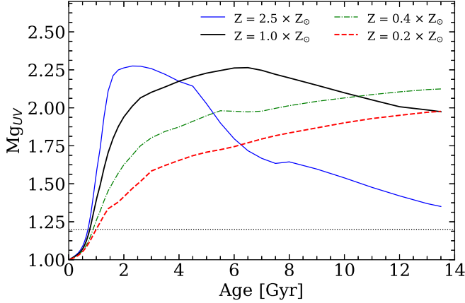
Fig. 2. Evolution of the strength of the M_{\text{gUV}} index as function of time for four metallicities: Z_{\odot} (solar, black solid line), 0.2 \times Z_{\odot} (red dashed line), 0.4 \times Z_{\odot} (green dot-dashed line), and 2.5 \times Z_{\odot} (solid blue line). The index is computed from SEDs created from the BC03 models (Bruzual & Charlot 2003) with an exponentially delayed SFH with an e-folding time of 0.1 Gyr and no dust extinction. The index was computed directly on the synthetic spectra.
