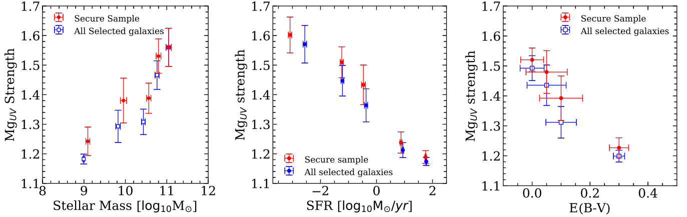
Fig. 6. Relationship between physical parameters computed from the SED-fitting based on photometric data only and the strength of Mg_{UV} computed from the SED-fitting of the spectroscopic data only. From left to right: stellar mass, SFR, and dust extinction. The errors shown on each plot represent the errors on the mean. In each panel we give the evolution for the full sample of 103 galaxies (blue) and also the evolution for the secure sample only (75 galaxies, in red).
