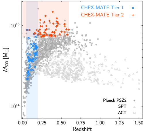
Fig. 5. Distribution in the M_{500} - z plane of confirmed clusters from major SZE surveys, available at the time of proposal submission (October 2017). Adapted from CHEX-MATE collaboration (2021).
