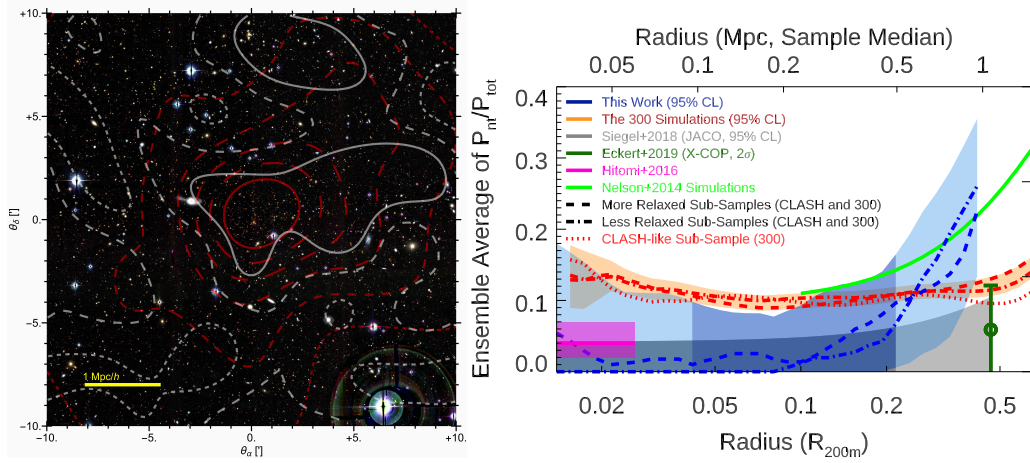
Fig. 4. (Left) Adapted from Sereno et al. (2018). Colour image of the region around PSZ2 G099.86+58.45. The contours show the mass distribution reconstructed from WL (white), and optical i -light of the galaxies with photometric redshift within \pm 0.06(1+z) of the cluster redshift (red). The longer the dash, the higher the contour value. The map is centred on the Brightest Cluster Galaxy. North is up. (Right) Adapted from Sayers et al. (2021). Ensemble-average P_{nt}/P_{tot} from the analysis of 16 CLASH galaxy clusters. Lighter shading indicates regions where biases due to modeling systematics may exist. Dashed and dot-dashed lines indicate the most likely profiles for the more relaxed and less relaxed sub-samples of the CLASH galaxy clusters and the 300 simulations. The red dotted line shows the most likely profile from a CLASH-like selection of 20 objects from the 300 simulations.
