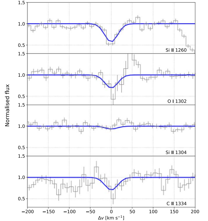
Figure 6. Transitions detected at z = 7.368 in the X-Shooter spectrum of ULAS J1342+0928. The lines are the same as in Figure 5. This figure can be compared with Figure B.59 in Christensen et al. (2023), noting the different velocity scale.
