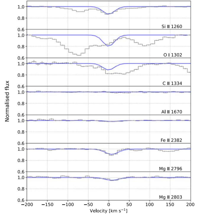
Figure 5. Transitions detected at z = 6.2897 in the X-Shooter spectrum of UHS J0439+1634. The observed flux is plotted as a gray histogram with 1\sigma error bars plotted for each pixel; the Voigt profile model is plotted as a blue solid line. This figure can be compared with Figure B.45 in Christensen et al. (2023), noting the different velocity scale.
