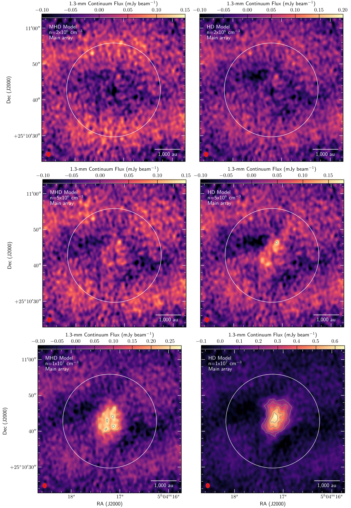
Figure 10. Simulated ALMA Main Array observations of the cores in Figure 7, with MHD simulations in the left panel and HD simulations in the right panels. Significant emission is only found when the central densities are 1 \times 10^7 \text{ cm}^{-3} , due to the fact that at lower central densities the dense cores have smooth and large inner kernels, which are filtered out by the Main Array. In the panels with detections, contours start at 5\sigma and are in steps of 3\sigma (with \sigma = 36 \mu\text{Jy beam}^{-1} ). The white circle is the primary beam and the red ellipse in the bottom left corner is the synthesized beam.
