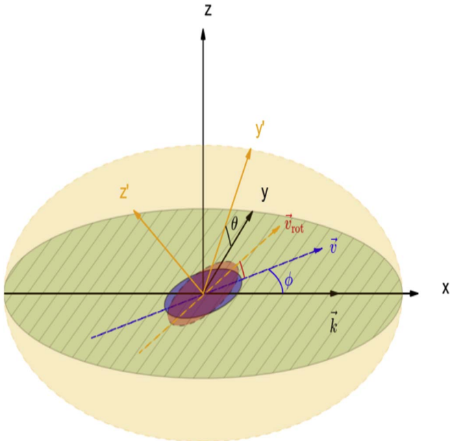
Figure 9. Illustration of the rotation of the elongated kernel around axis \mathbf{k} . The green shaded region represents the original ellipsoid before tilting, and orange represents the ellipsoid after tilting by angle \theta . The original elongated kernel with a major axis along \mathbf{v} is hence rotated into the kernel with major axis \mathbf{v}_{\text{rot}} . Such a misalignment will disappear if \mathbf{v} or when the kernel has an axis ratio similar to that of the larger oblate core.
