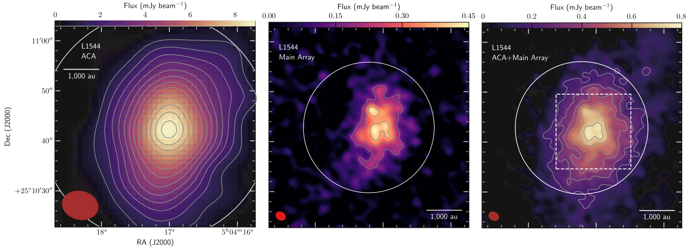
Figure 1. 1.3 mm dust continuum emission toward L1544 as seen by: (left) the ACA, with contours starting at 5\sigma (with \sigma = 0.21 \text{ mJy beam}^{-1} ) in steps of 3\sigma ; (center) the 12 m array only, with contours starting at 5\sigma (with \sigma = 34 \mu\text{Jy beam}^{-1} ) in steps of 3\sigma ; and (right) combined ACA+12 m array, with contours starting at 5\sigma (with \sigma = 36 \mu\text{Jy beam}^{-1} ) in steps of 3\sigma . The white dashed square is the area shown in Figure 2. The white circles in the three panels represent the corresponding 50% primary beam response. The red ellipses in the bottom left of the three panels are the synthesized beams.
