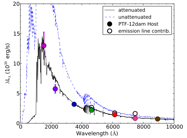
Figure 6. The best-fit ( \chi^2 = 1.3 ) SED of the host galaxy of PTF12dam from MAGPHYS (da Cunha, Charlot & Elbaz 2008), with (black line) and without (blue line) an attenuation by internal dust. The solid circles show the photometry from the galaxy continuum component, in the order of GALEX FUV , NUV and SDSS ugriz filter regions. Since there are no strong emission lines in FUV , NUV , u and z bands, we only removed the emission line contributions in gri bands. The hollow circles show their original photometric values of the host including emission line flux.
