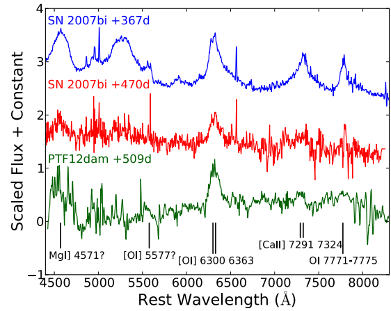
Figure 5. Spectrum of the host galaxy of PTF12dam at +508.6d taken by GTC. Comparison with the late-time spectra of SN 2007bi from the WIS-eREP database (Yaron & Gal-Yam 2012), which were published on Young et al. (2010); Gal-Yam (2012). Both wavelength and phases are stated in the SN rest-frame.
