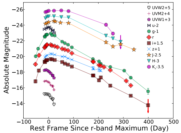
Figure 4. Absolute lightcurves of PTF12dam. Photometric points after +230d were based on this work applying for the proper host subtraction; before +230d were taken from Nicholl et al. (2013). Upper limits are shown with arrows of r and K_s bands at the last epochs. All points have been corrected for extinction, and griz magnitudes have also been K -corrected.
