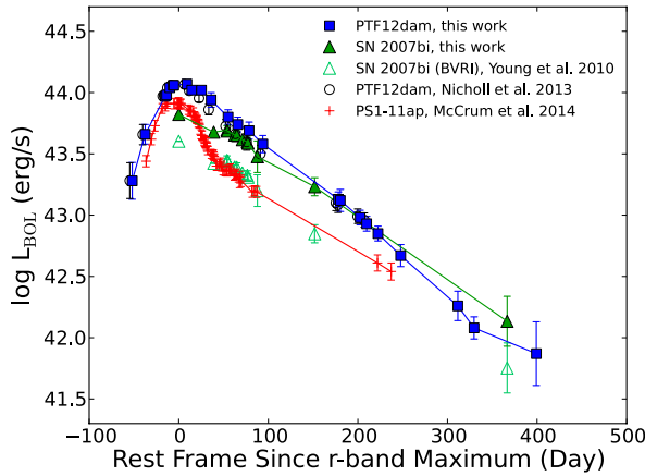
Figure 8. Bolometric lightcurves of PTF12dam, SN 2007bi and PS1-11ap. A true bolometric lightcurve of PTF12dam (integrating the estimated SED from the FUV to MIR) is shown as the solid blue squares. For reference, the previously published calculations of Nicholl et al. (2013) are plotted and the differences are discussed in section 4. A similar, true bolometric lightcurve of SN 2007bi is shown using the BVRI broad band photometry from Young et al. (2010) and a similar SED evolution as for PTF12dam. For comparison the pseudo-bolometric lightcurve presented in Young et al. (2010) is plotted, indicating what the likely correction is if flux in the UV and NIR/MIR is ignored. The bolometric lightcurve of PS1-11ap as calculated in McCrum et al. (2014) is plotted as red crosses. This is directly comparable with the true bolometric lightcurves of PTF12dam and SN 2007bi, although beyond +100-150d it may be underestimated by 10-20% due to lack of inclusion of a MIR contribution.
