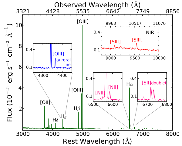
Figure 2. Spectrum of the host galaxy of PTF12dam. The [O III] \lambda 4363 auroral line and the region near H \alpha are amplified. The NIR spectrum taken from Nicholl et al. (2013) is shown in the upper-right panel.
