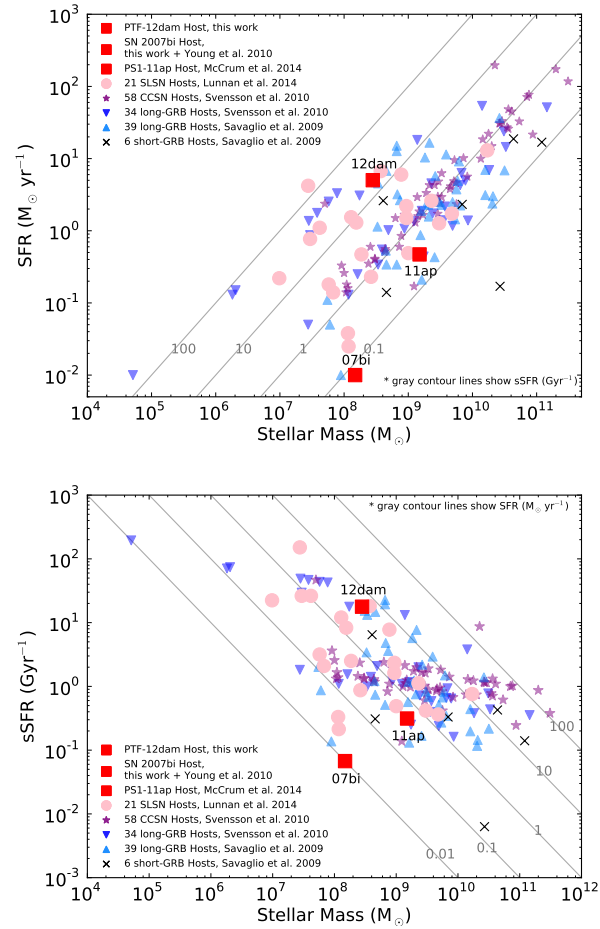
Figure 12. Stellar mass vs. star-formation rate (top) and specific star-formation rate (bottom) for SLSNe Ic (Lunnan et al. 2014), GRB (Savaglio, Glazebrook & Le Borgne 2009; Svensson et al. 2010) and CCSN hosts (Svensson et al. 2010). The three red boxes show the locations of the three slowly fading SLSNe Ic published to date (Young et al. 2010; McCrum et al. 2014).
