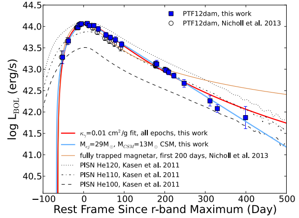
Figure 10. Bolometric lightcurve of PTF12dam and alternative models. The new bolometric lightcurve of PTF12dam is shown with blue squares and the new magnetar best-fit model with \kappa_{\gamma} = 0.01 \text{ cm}^2 \text{ g}^{-1} is the red line. For comparison, the black circles show the bolometric lightcurve of PTF12dam from Nicholl et al. (2013), and their fully trapped magnetar model ( \kappa_{\gamma} = \infty ) is shown by the orange line. Background black lines illustrate PISN models (Kasen, Woosley & Heger 2011) of different mass, which are not fitted with the PTF12dam lightcurve evolution. Our CSM model (blue line) is also present. See section 5 for details.
