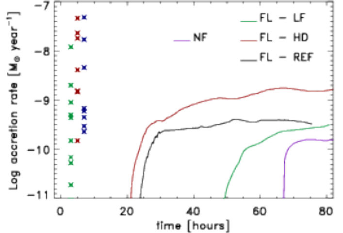
Fig. 8. Evolution of accretion rates synthesized from runs FL-REF (black line), FL-HD (red line), FL-LF (green line), and NF (purple line). The crosses represent the values of mass accretion rates inferred from optical-near UV observations for a sample of low-mass stars and brown dwarfs (green, Herczeg & Hillenbrand 2008 ), for a sample of solar-mass young accretors (red, Herczeg & Hillenbrand 2008 ), and for an X-ray-selected sample of CTTSs (blue, Curran et al. 2011 ); their position on the time axis is chosen to facilitate comparison with the model results.
