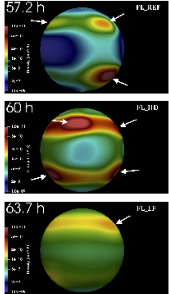
Fig. 9. Maps of particle number density in log scale close to the stellar surface after about 60 h of evolution for runs FL-REF (upper panel), FL-HD (middle panel), and FL-LF (lower panel). The high-density regions (pointed at by white arrows) correspond to accretion columns impacting onto the stellar surface. Runs FL-REF and FL-HD exhibit clear hotspots, whereas in run FL-LF, the matter is more diffused and the contrast in density is weaker.
