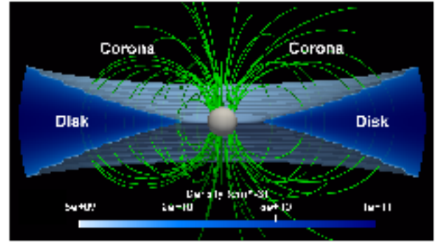
Fig. 1. Initial conditions for the reference case. In blue we present in logarithmic scale the density map of the disk, the green lines show the sampled magnetic field lines, and the white sphere represents the stellar surface that marks a boundary.
