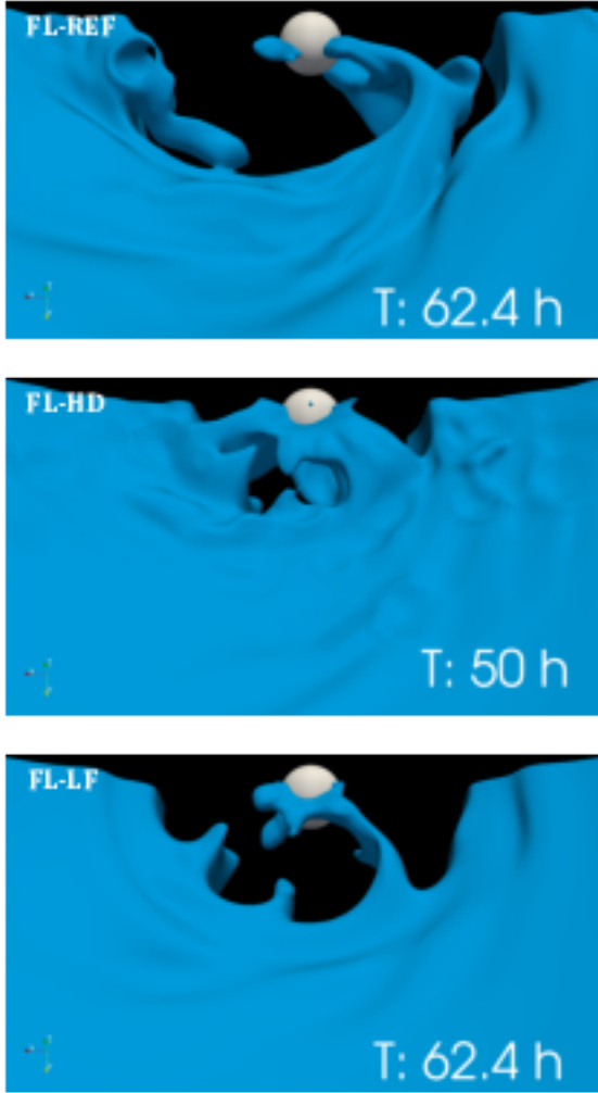
Fig. 7. Representative close up views of the inner region of the star-disk system for runs FL-REF (top panel), FL-HD (middle panel), and FL-LF (bottom panel). In blue we show the isosurfaces where the disk material has a particle number density n = 10^{10} \text{ cm}^{-3} . The white sphere in each panel represents the stellar surface.
