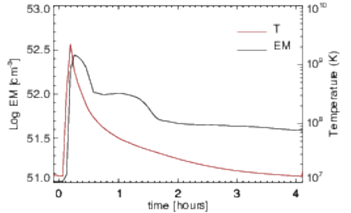
Fig. 3. Evolution of the maximum temperature (red line) and integrated EM (black line) of the plasma with \log(T) > 6.3 for the second flare in run FL-REF. The initial time is at the release of the corresponding heat pulse.
