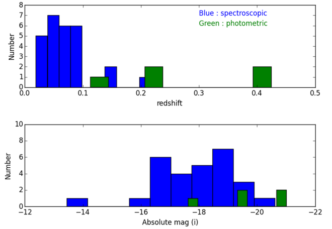
Figure 5. Histograms of the redshift distribution and absolute magnitudes ( M_{iP1} ) of the confirmed SN or likely SN transients. The objects in blue either have a spectroscopic redshift from the transient itself, or host galaxy. The objects in green have a photometric redshift of the host galaxy from SDSS DR12. The AGN/QSO candidates are not included. All magnitudes are in i_{P1} apart from one (PS15ckf) which is in z_{P1} .
