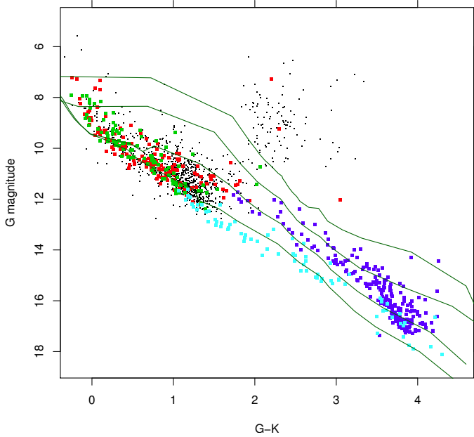
Fig. 6. (G, G - K) Colour-magnitude diagram. Symbols are the same as in Fig. 4, with the addition of stars from Jeffries et al. (2014 – blue) and Sacco et al. (2015 – cyan). Shown are isochrones from Siess et al. (2000 – dark green), at ages of 1, 3, 10, and 30 Myr, at zero reddening and distance of 356 pc.
