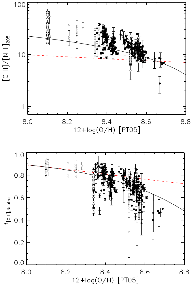
Figure 4. Top: the ratio of [C\ II]/[N\ II]_{205\ \mu m} as a function of gas-phase oxygen abundance. Bottom: the fraction of [C\ II] emission originating in the neutral phase plotted as a function of the metallicity, assuming C/N_{\odot} . Regions in galaxies for which Moustakas et al. (2010) determined a gradient are plotted as filled points while open points indicate global O/H measurements. The black lines represent a fit to f_{[C\ II], Neutral} and the linear O/H ratio, while the dashed red lines show the arbitrarily normalized, modest trends expected if the [C\ II] neutral fraction were in fact fixed, and changes in [C\ II]/[N\ II]_{205\ \mu m} and f_{[C\ II], Neutral} were driven solely by underlying C/N variation with 12+\log(O/H) as expressed in Equation (2). The O/H abundance is on the scale of Pilyugin & Thuan (2005).
