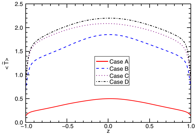
Figure 1. Horizontally and time-averaged profiles of the temperature as functions of z for the cases A–D with zero net flux and different aspect ratios. The corresponding averaged surface heat fluxes for cases A–D are, respectively, 0.012, 0.18, 0.26, and 0.29.
