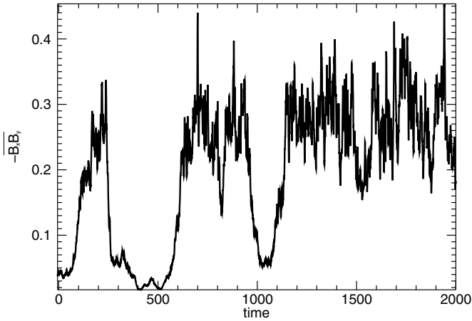
Figure 5. Time history of the Maxwell stresses averaged over the computational box for case D. The time history covers the full simulation length of 2000 time units.
