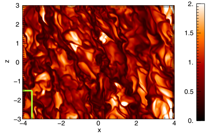
Figure 4. Typical temperature planform at the upper boundary of the computational box for case D with zero net flux and the largest aspect ratio. The green rectangle in the lower left corner of the figure shows the extent of the computational grid for case A.
