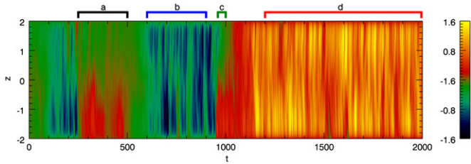
Figure 6. Space-time diagram of the average azimuthal field for case D. The horizontally averaged value of B_y is plotted as a function of z and t . The diagram covers the full simulation length of 2000 time units. Above the diagrams we have marked four time intervals, denoted by the letters a, b, c, and d, during which we have alternatively low and high states. The time-averaged vertical profiles of azimuthal field shown in Figure 7 refer to these four time intervals.
