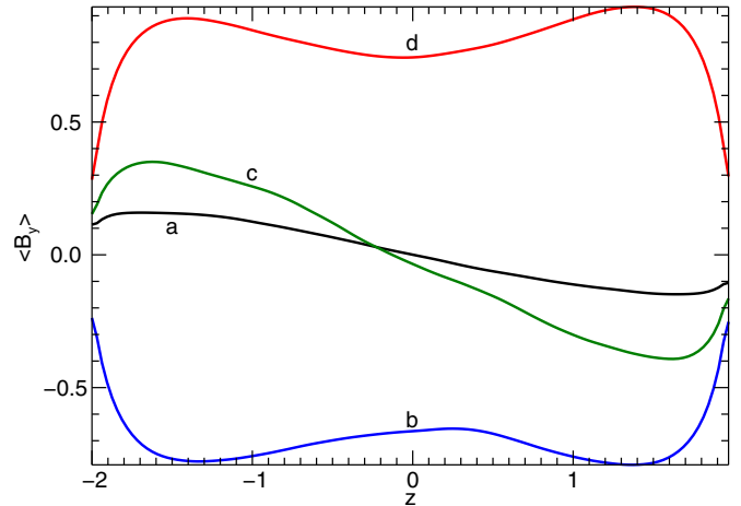
Figure 7. Vertical profile of the time-averaged azimuthal field as functions of z . The four curves refer to the four time intervals—a, b, c, and d—marked in Figure 6, for which we have alternatively low and high states.
