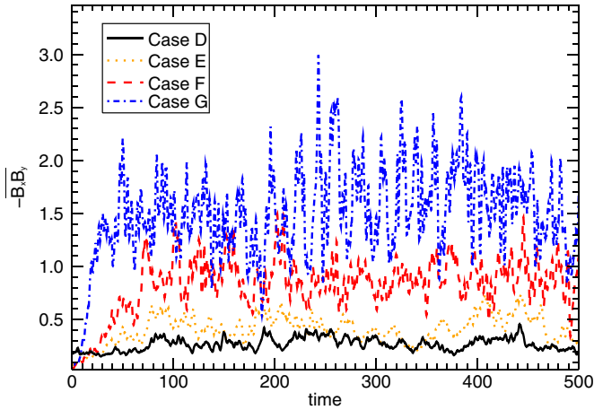
Figure 9. Time histories of the Maxwell stresses averaged over the computational box for the cases E–G with net magnetic flux and different initial vertical field strengths. For comparison, we also show case D with zero net flux and the same aspect ratio.
