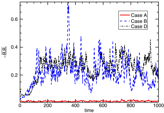
Figure 2. Time histories of the Maxwell stresses averaged over the computational box for the cases A, B, and D with zero net flux and different aspect ratios. The time history for case D covers the second half of the simulation, the full time history for this case is shown in Figure 5.
