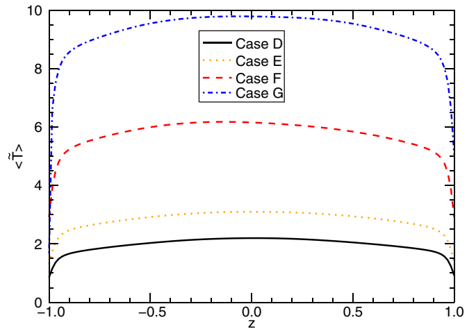
Figure 8. Horizontally and time-averaged profiles of the temperature as functions of z for the cases E–G with net magnetic flux and different initial vertical field strengths. For comparison, we also show case D with zero net flux and the same aspect ratio.
