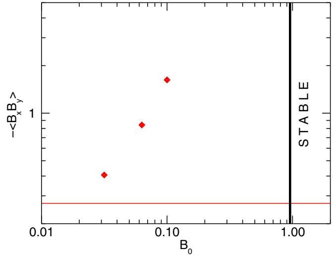
Figure 11. Box and time-averaged values of the Maxwell stresses for cases E–G as a function of the initial vertical field strength B_0 . The horizontal line corresponds to the average stress value for case D with zero net flux in the high state. The vertical line shows the linear stability boundary for a state with constant density.
