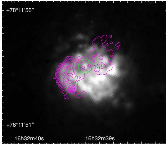
Figure 5 The HST H\alpha image of the central 7'' \times 7'' , corresponding to 680 \times 680 pc, nuclear region in NGC 6217, overlaid with the radio contours from the combined e-MERLIN/VLA data in magenta. The radio contours are set at 50, 100, 150, 200, 300, 400, 500 \times 10^{-6} \text{ Jy beam}^{-1} . The green circle is centred on the hottest pixel in the H\alpha image and the radius corresponds to the typical HST \sigma of 0''.3 . North is up and east is to the left.
