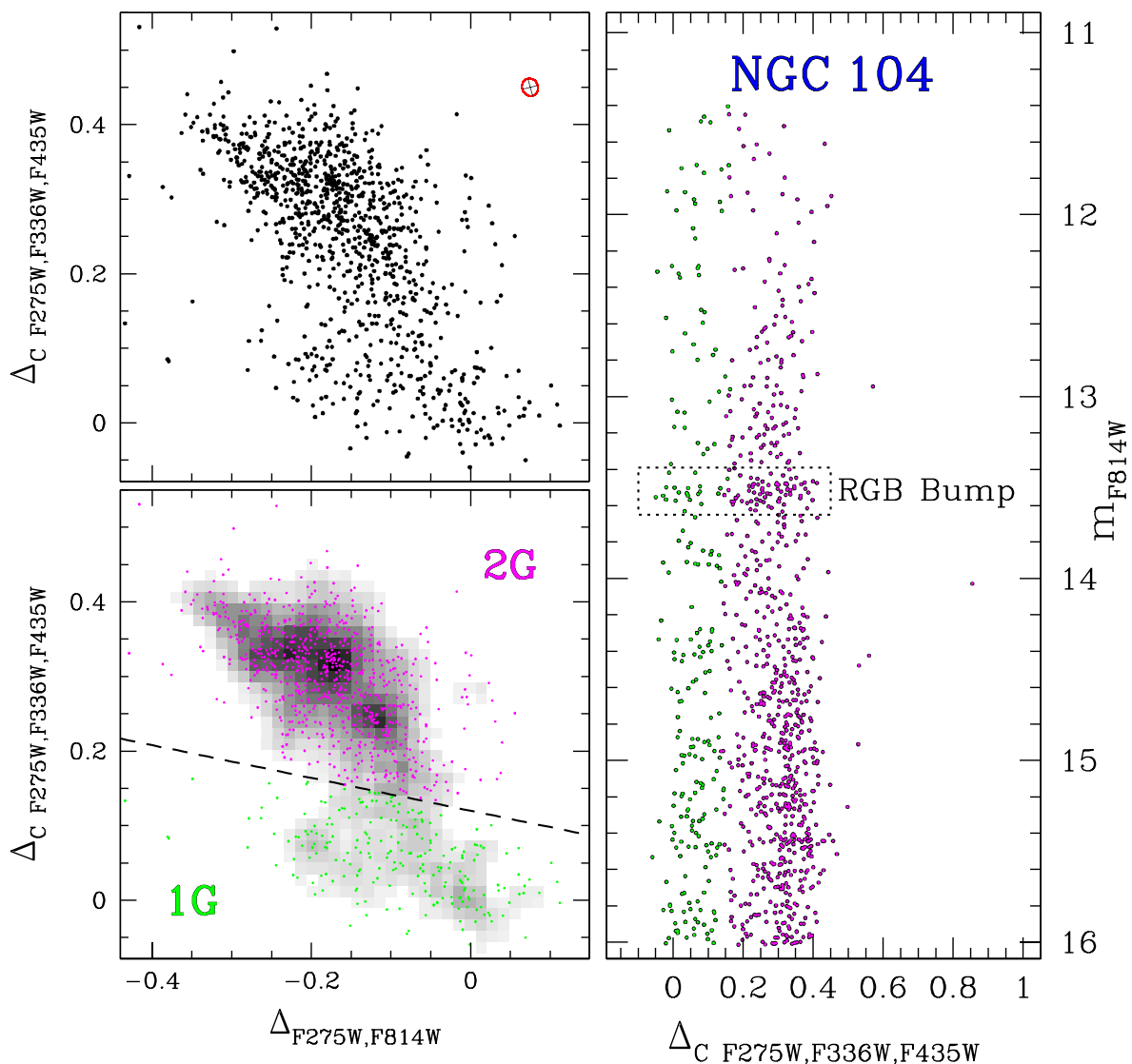
Figure 1. Upper-left panel: \Delta_C F275W, F336W, F435W versus \Delta_F275W, F814W diagram (chromosome map) of the RGB stars of the GC NGC 104. The red ellipse marks the 68.27th percentile of the expected distribution of the observational errors in this diagram (see Paper IX). Lower-left panel: stellar density diagram relative to the chromosome map. The black dashed line divides the first (1G) and second (2G) stellar population in the chromosome map. 1G and 2G stars have been plotted over the density diagram as green and magenta dots, respectively. Right-hand panel: m_{F814W} versus \Delta_C F275W, F336W, F435W diagram of the cluster RGB. The dotted box indicates the approximate position of the 1G and 2G RGB bump stars.
