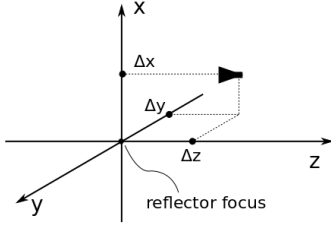
Figure 3. Geometry of the feed displacement.
