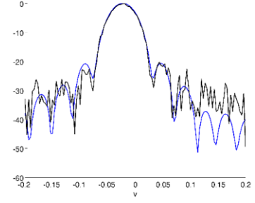
Figure 8. Cut along the v -axis of the normalized amplitude (dB) of the reconstructed FFP on the standard grid. The black line represents the far-field data while the blue line represents the reconstructed field.
