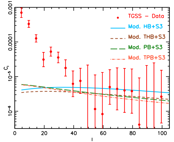
Fig. 10. As in Fig. 9 but for the TGSS sample. The measured APS (red dots) is compared to model predictions (continuous curves with different line styles).
