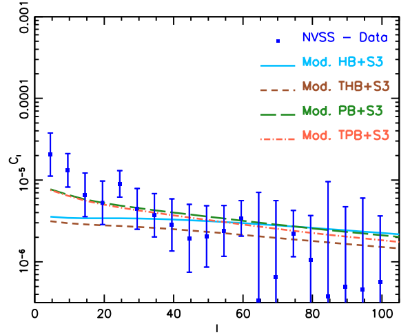
Fig. 9. Measured NVSS APS (blue squares from Fig. 5) vs. model predictions. The different models are listed in Table 2 and described in the text, and represented with different line styles, as indicated in the plot.
