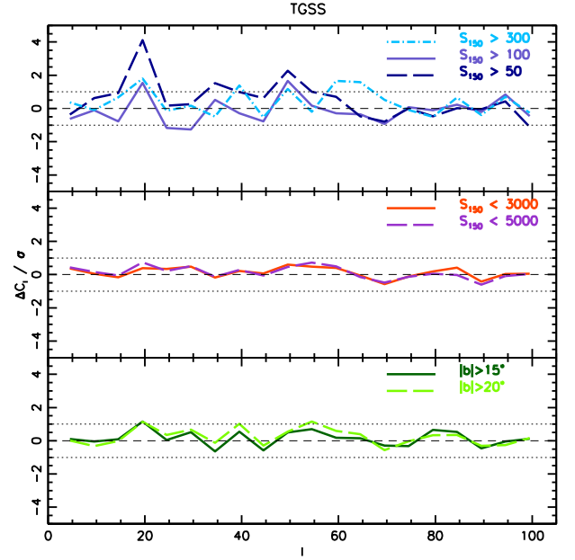
Fig. 6. Angular power spectrum residuals of different TGSS samples with respect to the Reference case, expressed in units of Gaussian errors. Upper panel: normalized residuals of the TGSS samples selected at different values of the minimum flux cut, \underline{S}_{150} , indicated in the plot, compared to the Reference case of \underline{S}_{150} = 200 mJy. Middle panel: we consider samples selected at different values of the maximum flux cut, \bar{S}_{150} ; the Reference is \bar{S}_{150} = 1000 mJy. Bottom panel: residuals for samples with different geometry masks, cut at different values of the Galactic latitude, also indicated in the plot, referred to the baseline case of |b| > 10^\circ . The dotted horizontal lines in all panels indicate the 1\sigma Gaussian error of the Reference sample. The dashed horizontal line indicates the zero residual level.
