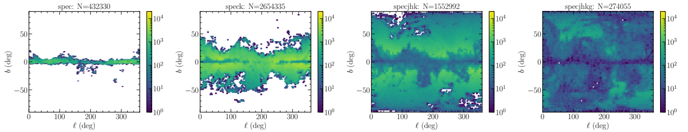
Fig. 7. Spatial distribution, in galactic sky-coordinates ( \ell, b ), of the number of stars for which we adopt each projection flavour. The total of selected stars and the considered projection are indicated at the top of each plot. Only targets with GSP-Spec KMgiantPar_flag= 0 are considered here.
