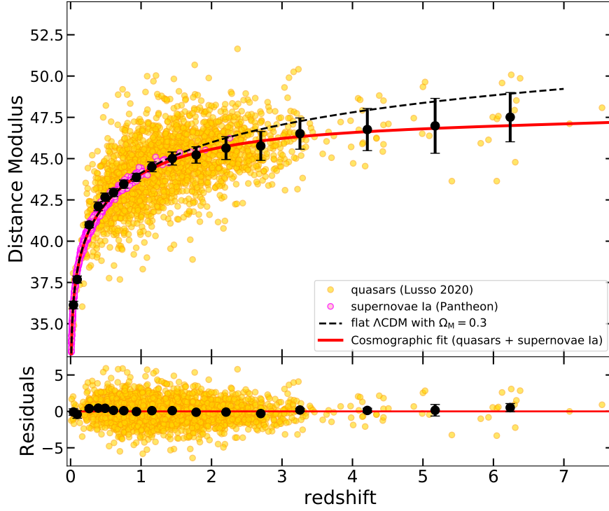
Fig. 14 Hubble diagram of QSOs [182] and SNe Ia [Pantheon 189, magenta points]. The red line represents a fifth order cosmographic fit of the data, whilst the black points are averages (along with their uncertainties) of the distance moduli in narrow (logarithmic) redshift intervals. The dashed black line shows a flat \Lambda CDM model fit with \Omega_M = 0.3 . The bottom panel shows the residuals with respect to the cosmographic fit and the black points are the averages of the residuals over the same redshift intervals. Figure adapted from [182].
