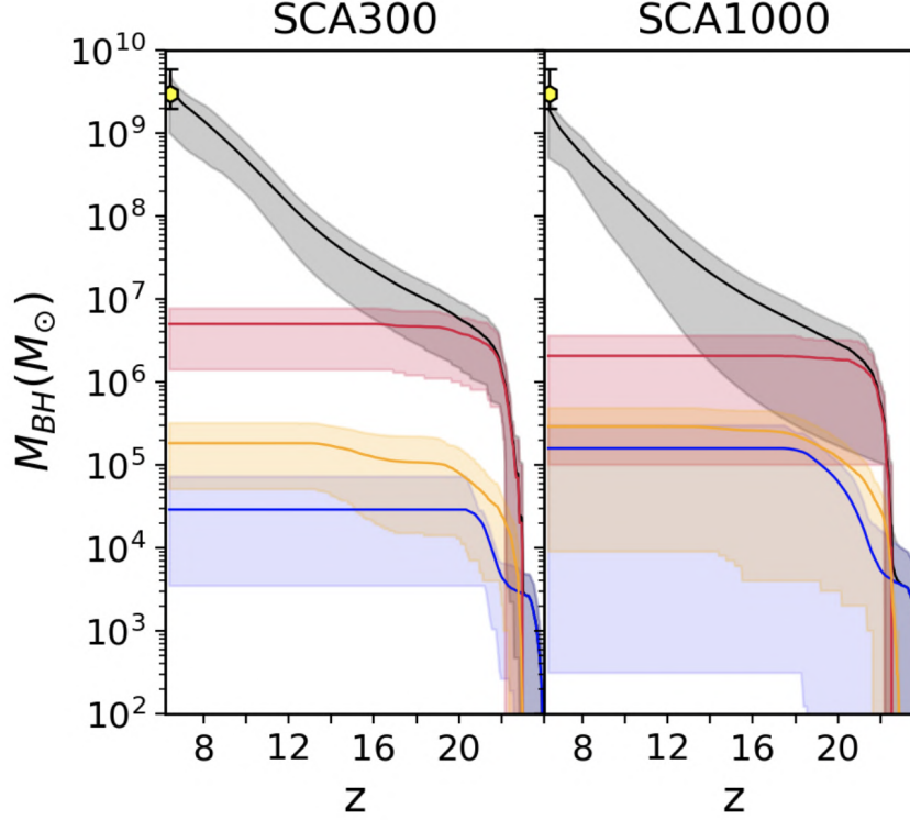
Fig. 5 Redshift evolution of the SMBH powering a z > 6 QSO via Eddington-limited gas accretion and mergers with other BHs (black line), in the SCA scenario (see Section 3.2 and [74] for details). The blue, yellow and red lines instead show the relative contribution, without gas accretion, of light, medium-weight, and heavy BH seed progenitors, respectively. Each curve is obtained averaging on 10 different merger tree realisations of the 10^{13} M_{\odot} QSO host halo, and the shaded areas bracket the minimum and maximum mass reached at each redshift. The two panels are for two different critical LW radiation threshold J_{\text{cr}} = 300 (left panel) and J_{\text{cr}} = 1000 (right panel). The data point at z = 6.4 indicates the estimated SMBH mass of the QSO SDSS J1148+5251 assumed as a prototypical system and against which the model parameters have calibrated. The figure is taken from [74].
