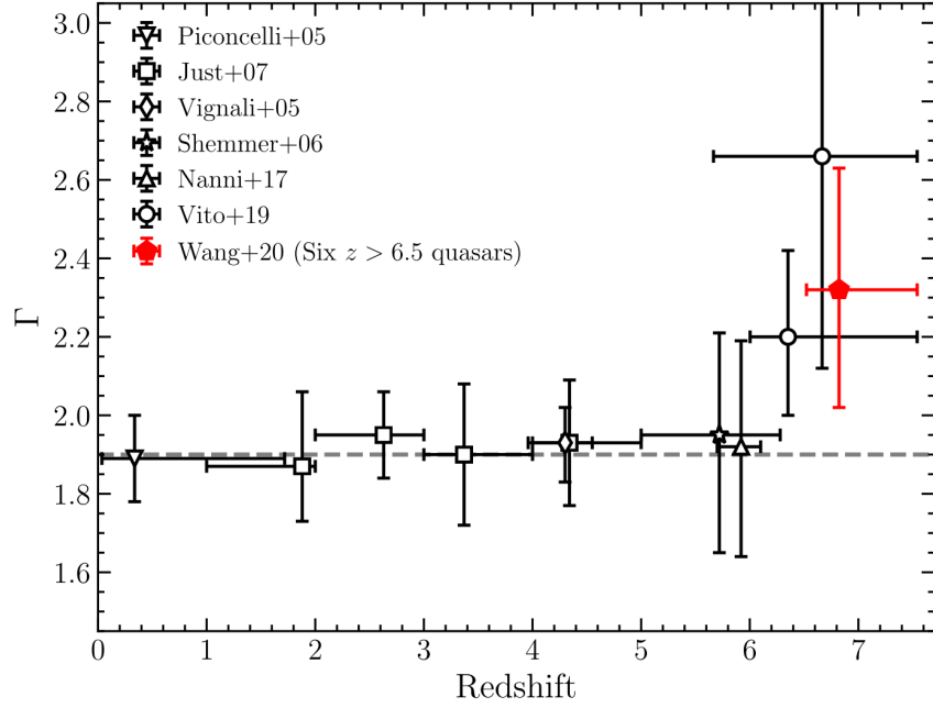
Fig. 12 Average photon index of optically selected QSOs as a function of redshift. From [132]. © AAS. Reproduced with permission.
