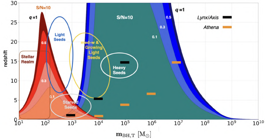
Fig. 18 Summary of the GW and EM landscape. The coloured curves are the sensitivity limits (also known as waterfall plots) showing the average GW horizon computed for S/N = 10 and mass ratios q = 1, 0.5, 0.3, 0.1 both in the ET (red) and LISA (blue) bandwidth [228, 229]. Thick horizontal bars indicate the sensitivity of the deepest pointing, in the [0.5 - 2] keV observed band, of the missions Athena (orange) and of the NASA concepts Lynx/Axis (black). Ellipses show where stellar-mass BHs (red), light (blue), medium-weight (yellow) and heavy (white) seeds are expected to form. In the yellow region newly formed medium-weight seeds and light seeds that grow in time via accretion and mergers are expected to co-exist. The transit to the SMBH domain covers the entire LISA area and EM observations are key to discover the high-mass tail of the SMBH distribution. The light-grey ellipse at z \leq 5 marks the population of long-living “starved” merging seeds (i.e. seeds whose growth is stunted by several processes) that could be detectable at late times when merging with other SMBHs at z \leq 5 ([114]). The gap in the deci-Hz window, between the ET and LISA domain, is the territory of decihertz GW observatories/programs like DECIGO and AION. Figure adapted from [114].
