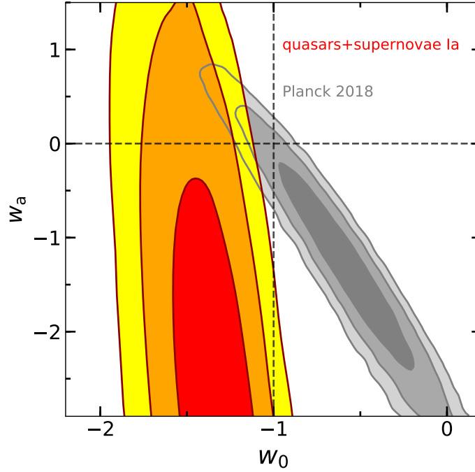
Fig. 15 Marginalized posterior distributions (1, 2 and 3\sigma ) of the (w_0, w_a) parameters for the combined QSOs [182] and SNe Ia [189] samples (red-orange-yellow contours). The constraints from the combination of Planck TT,TE,EE+lowE+lowl (i.e. baseline parameter analysis) with the inclusion of baryonic acoustic oscillations are also shown [grey contours 190]. The dashed lines mark the point corresponding to the \Lambda CDM model. The resulting (w_0, w_a) for the combined QSOs + SNe are statistically consistent with the phantom regime ( w > -1 ) and at variance with the \Lambda CDM model at more than the 3\sigma statistical level. Image adapted from [191].
