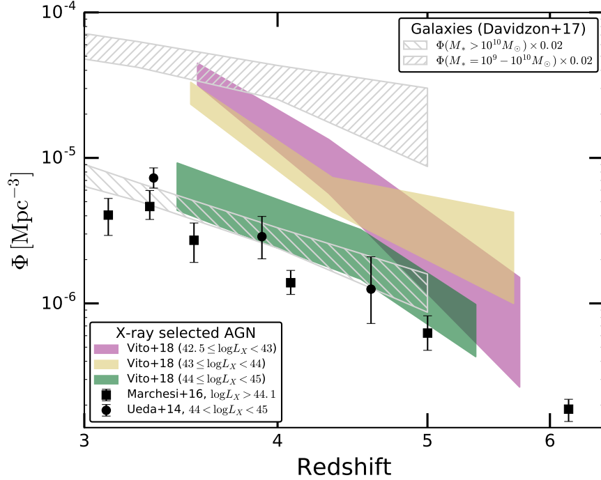
Fig. 16 Evolution of the space density of X-ray selected AGN with different luminosities at z = 3 - 6 (from [214, 207, 208]), compared with the space density of galaxies (from [215]) with different stellar masses (rescaled by a factor of 0.02).
