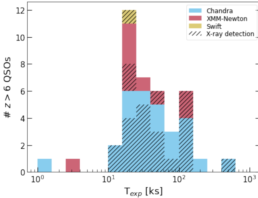
Fig. 7 Histogram of the exposure times of published X-ray observations of z > 6 QSOs (see Tab. 1). Blue, red, and yellow colours refer to observations performed with the Chandra , XMM-Newton , and Swift observatories, respectively. Detected sources are marked with hatching patterns.
