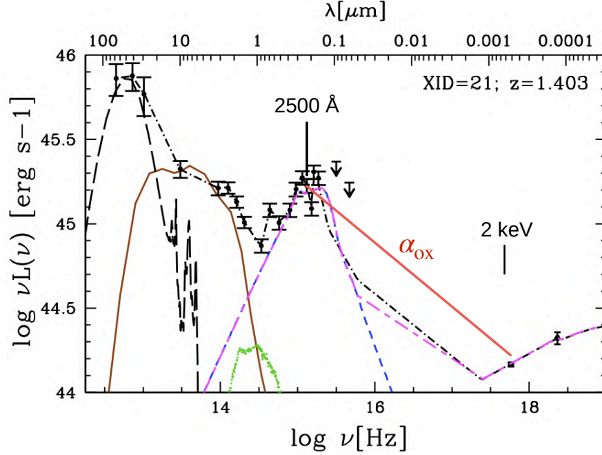
Fig. 13 Example of full AGN SED from far-IR to X-rays at redshift 1.4 from the XMM-COSMOS survey. The rest-frame data, used to construct the total SED (shown with a black dot-dashed line), are represented with black points. Various lines represent the different models adopted to describe the data. Specifically, the black long-dashed, brown solid, green dotted, and blue dashed lines correspond to the best-fit starburst, hot-dust from reprocessed AGN emission, host-galaxy, and the empirical disc templates, respectively. The magenta short-long dashed line is the best-fit empirical disc template with the inclusion of X-rays. The rest-frame 2500 Å and 2 keV are marked, as well as a representation of the \alpha_{\text{OX}} index for this object. This figure is adapted from [188].
