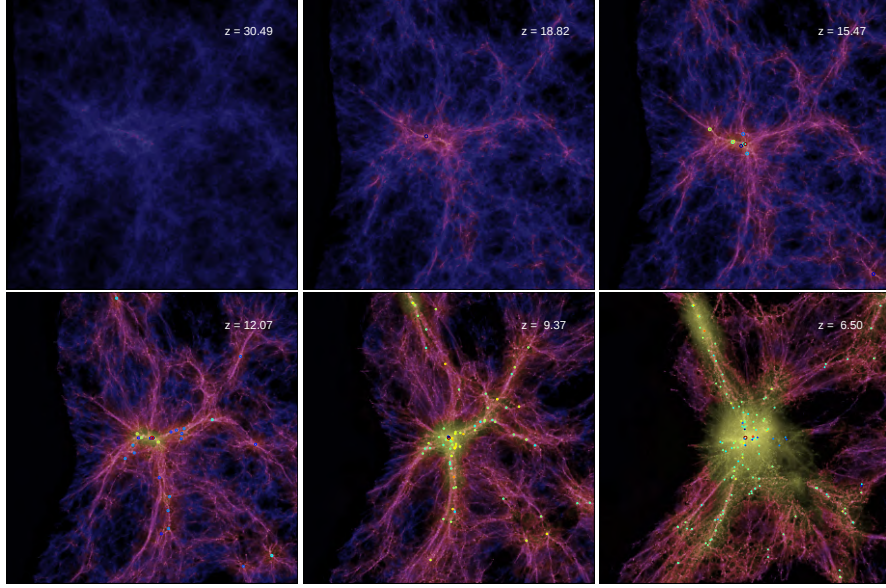
Fig. 4 Cosmological zoom-in simulation from [85]. The different images (snapshots) show the evolution of the first galaxies and BHs from z \sim 30 to z \sim 6.5 , simulated within a zoom-in region of 10 comoving Mpc size centred on a 10^{13} M_{\odot} dark matter halo. Each snapshot shows the projected gas density colour-coded with temperature: cold gas is in blue while the hot gas (heated and ionised by SN and accreting BH feedback) is represented in yellow. In this model the author assume that a seed BH of \sim 10^5 M_{\odot} is planted with halos of \sim 10^{10} M_{\odot} and subsequently grows via Eddington-limited chaotic accretion assuming the standard, thin-disc accretion model. Coloured circles indicate the locations of BHs.
