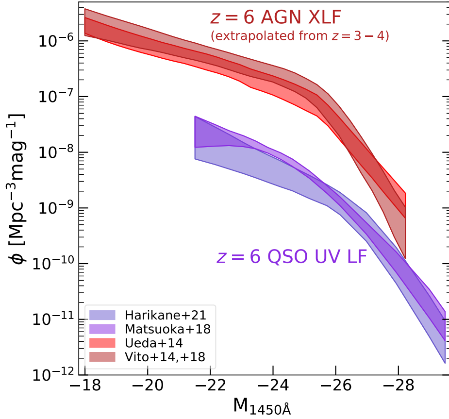
Fig. 17 Comparison between the UVLF (from [199, 218]) and XLF (from [214, 206], extrapolated and transformed into UVLF as described in the text) of z \approx 6 QSOs. The different normalizations suggest the existence of \approx 90\% QSOs missed by UV selection, most probably due to obscuration.
