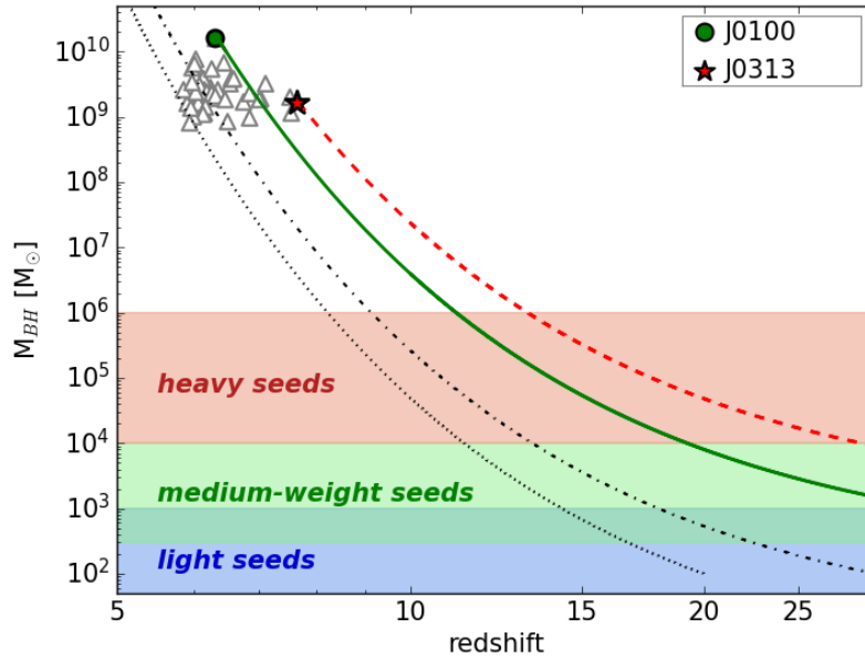
Fig. 2 Black hole growth tracks for a sample of z > 6 QSOs. To prepare this figure, BH masses have been consistently re-calculated using the same virial estimator, based the observed MgII 2798 Å emission line (mass calibration from [66]). The dotted and dot-dashed lines show the time evolution of a light seed of 100 M_{\odot} forming at z = 20 and z = 30 , respectively. The remaining curves instead give the mass of the seed required to grow the final observed SMBH in J0100 (green solid) and J0313 (red dashed), in less than \sim 700 - 800 \text{ Myr} . In this figure each SMBH grows from a single seed that accretes gas at the Eddington rate ( \dot{M} = \dot{M}_{\text{Edd}} ) at all times. The three shaded areas approximately indicate the mass range of the different seed populations: light seeds (blue), medium-weight seeds (green) and heavy seeds (red).
