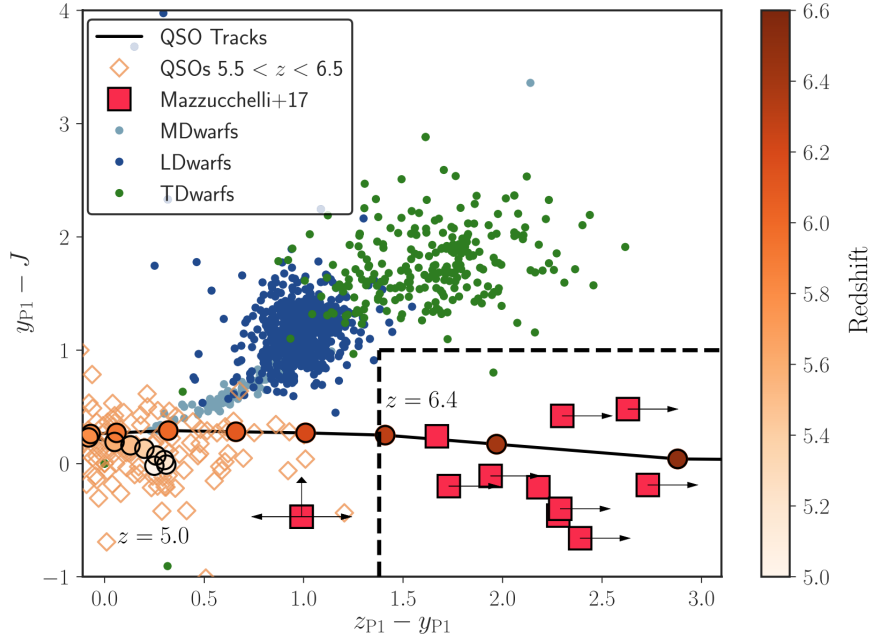
Fig. 6 Example of colour-colour diagram used to select high-redshift QSOs. The location of known 5.5 < z < 6.5 QSOs (open diamonds) and the expected colour track of a high-redshift QSO (black line and circles) are shown and colour-coded according to the redshift. Cyan, blue, and green circles show the location of cold stars. The dashed lines mark the colour cuts used to select a sample of z > 6.5 QSOs (red rectangles), exploiting the flux drop between the z and y bands. From [12]. © AAS. Reproduced with permission.
