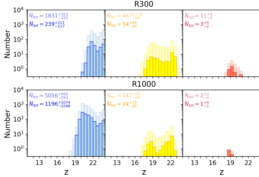
Fig. 3 Distribution of formation redshifts of light (left), medium-weight (middle), and heavy (right) BH seeds from [74]. The histograms show the mean values averaged over 10 different simulations of the host dark matter halo merger trees. Lighter colours show the global BH seed population, whereas histograms in heavier colours count only the progenitors of the final SMBH at z = 6.4 (i.e. those that are not ejected as satellite in minor halo mergers along the host galaxy cosmic assembly). Labels in each panel indicate the total number of seeds formed, on average, in the corresponding population. Corresponding upper and lower values indicate the difference with the maximum and minimum values for each family over 10 simulations. The top panels show the distribution of the reference model (R300) in which a critical LW flux level of J_{cr} = 300 is adopted. For comparison, the results obtained assuming a higher threshold, J_{cr} = 1000 are reported in the bottom panels (model R1000).
