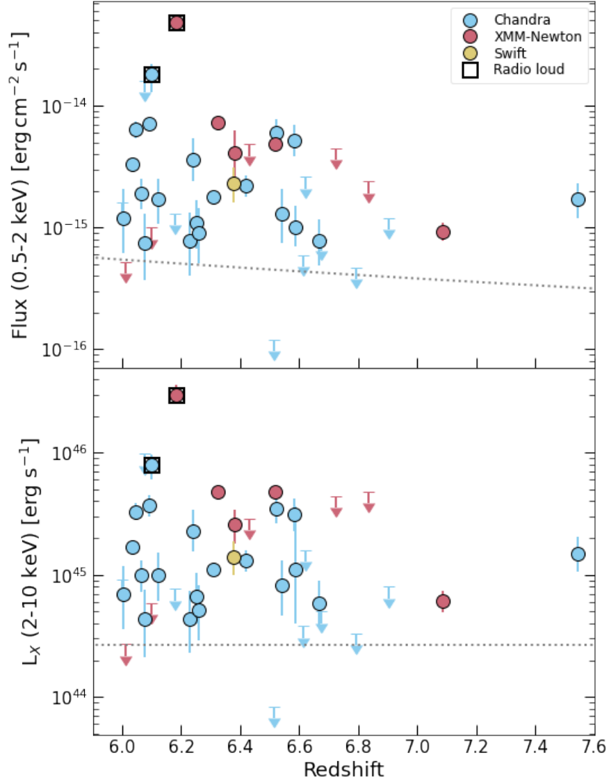
Fig. 8 Soft-band flux ( upper panel ) and 2–10 keV band luminosity ( lower panel ) versus redshift for z > 6 QSOs with published observations; see Fig. 7 for references. The dotted line marks the X-ray flux and luminosity corresponding to the knee of the z \approx 6 QSO UV luminosity function. The conversion assumes UV power-law emission f_\lambda \propto \lambda^{-0.3} ([5]), the \alpha_{\text{ox}} - L_{\text{UV}} relation of [143], and X-ray emission with \Gamma = 2 .
