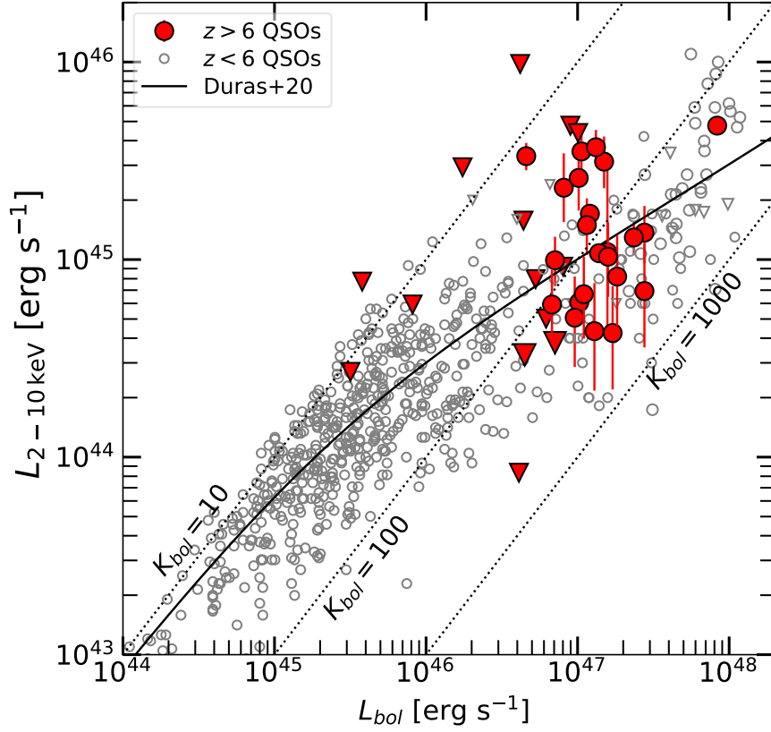
Fig. 11 X-ray luminosity vs. bolometric output of z > 6 QSOs (Tab. 1) compared with QSOs at lower redshift collected from [155, 134, 154, 157]. The black solid line is the best-fitting relation of [158]. The diagonal dotted lines marks loci of constant K_{\text{bol}} as defined in the text.
