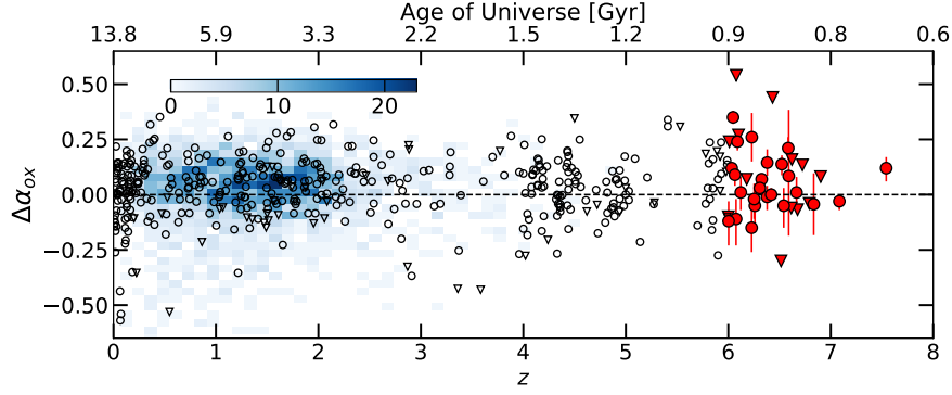
Fig. 10 \Delta\alpha_{\text{ox}} as a function of redshift. Symbols are as in Fig. 9. The values of \Delta\alpha_{\text{ox}} have been computed assuming the \alpha_{\text{ox}} - L_{\text{UV}} relation of [143].
