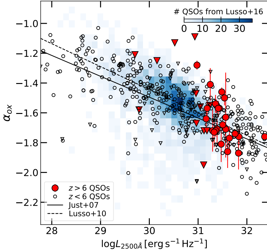
Fig. 9 \alpha_{\text{ox}} vs. UV luminosity of the high-redshift QSOs included in Tab 1 compared with the general QSO population (samples collected from [151, 152, 143, 153, 134, 154]). Only radio-quiet QSOs are considered. Downward-pointing triangles are upper limits. The solid and dashed lines are the best-fitting relations of [143] and [155].
