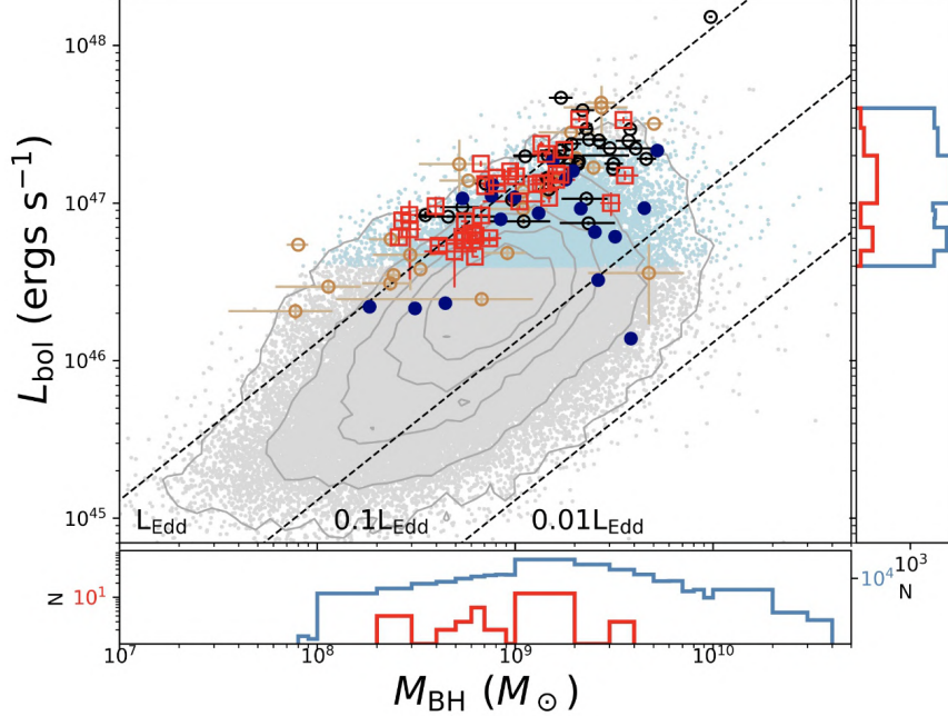
Fig. 1 Bolometric luminosities and black hole masses of a compilation of 6.0 \lesssim z \lesssim 7.6 QSOs (red, black, and brown symbols) compared with the SDSS lower-redshift ( 0.40 < z < 2.1 ) sample (grey dots). The light blue dots represent a sub-sample from the SDSS lower redshift survey with bolometric luminosity comparable to the highest-redshift sample presented by [1] (red). The right-hand and bottom histograms show the comparison of the luminosity and black hole mass distributions, respectively, in the two aforementioned samples, with the same colour-coding. The figures show that a large number of high-redshift QSOs are located close to (or above) the line of Eddington luminosity (upper dashed line). Figure is taken from [1]. ©AAS. Reproduced with permission.
