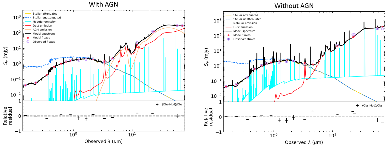
Figure 4. SED fitting of optical-IR photometric data of J1440 using the CIGALE software. The plots with AGN (left) and without AGN (right) are shown with its residual. The higher residual in the right panel suggests the need for an AGN component. Moreover, the AGN component in the optical band is heavily suppressed, which suggests the presence of an obscuring medium.
