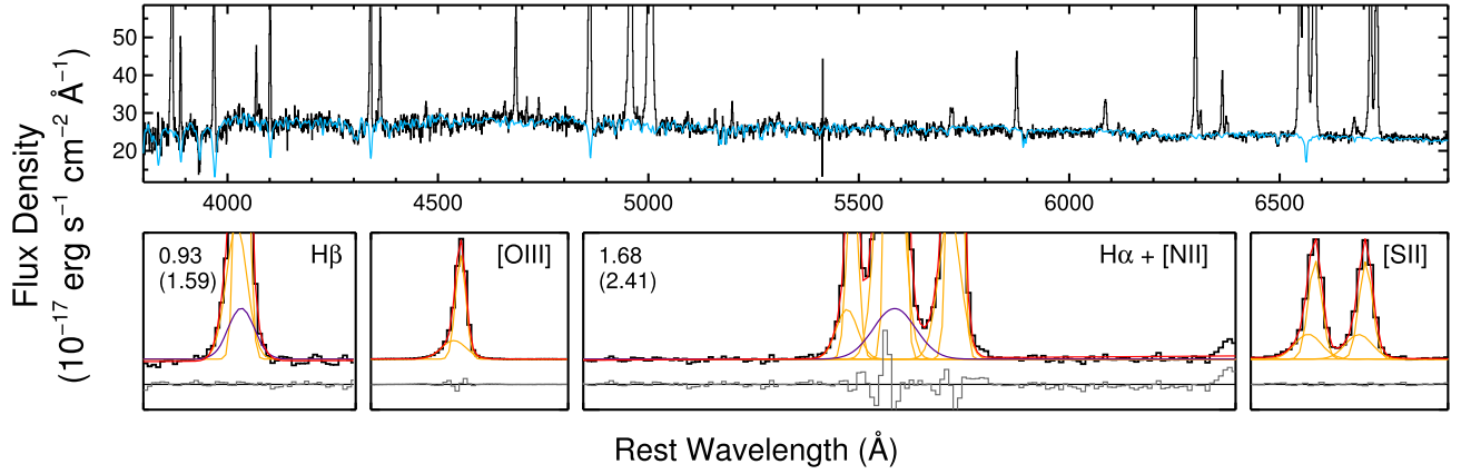
Figure 3. Optical spectrum for J1440 with zoomed-in line profile fits of key emission lines as analyzed in R13. The broad components in H \alpha and H \beta , as well as the strong [OIII] \lambda 5007 and [SII] lines, are indicative of AGN activities.
