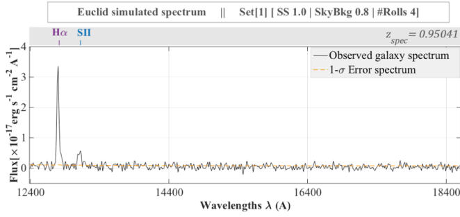
Fig. 15. Simulated Euclid spectra. Left : simulated galaxy spectrum (id: 53678850) in the dataset S1 with an identifiable H \alpha line at 12803A. Right : simulated galaxy spectrum (id: 56932048) in the dataset S2 with a H \alpha emission line at 12908A.
