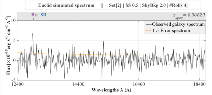
Fig. 15. Simulated Euclid spectra. Left : simulated galaxy spectrum (id: 53678850) in the dataset S1 with an identifiable H \alpha line at 12803A. Right : simulated galaxy spectrum (id: 56932048) in the dataset S2 with a H \alpha emission line at 12908A.
