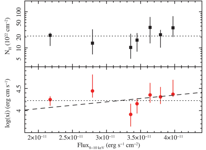
Figure 9. Best-fitting column density ( N_{\text{H}} , upper panel) and ionization parameter ( \xi , lower panel) of the photoionized plasma, as measured using the \text{zxipcf} spectral model, as a function of the observed 8–10 keV flux. No significant variation is observed in either of the two parameters (the dotted lines show a model with constant N_{\text{H}} and \xi ). The dashed line shows the best-fitting linear relation between ionization parameter and source luminosity.
