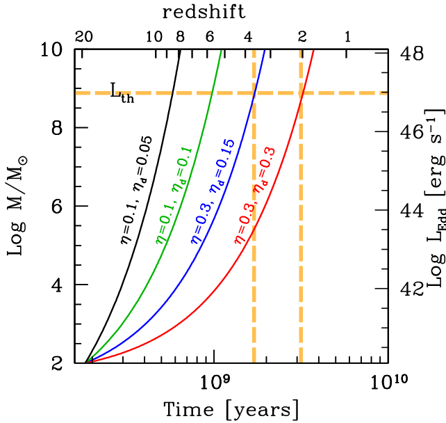
Figure 2. Growth of a black hole mass for different values of the total efficiency \eta and disc efficiency \eta_d . The horizontal dashed line corresponds to an assumed L_{th} = 10^{47} \text{ erg s}^{-1} . The vertical dashed lines correspond to the times (bottom axis) and the redshift (top axis) when the disc luminosity reaches L_{th} .
