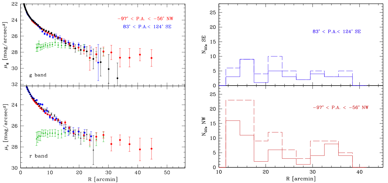
Figure 3. Left panel—SB profiles in the g (upper panels) and r bands (bottom panels), extracted in different areas around NGC 1399. Red circles: SB for -97^\circ \leq \text{P.A.} \leq -56^\circ , which covers the ICL region. Blue circles: SB for 83^\circ \leq \text{P.A.} \leq 124^\circ , which is the region opposite of the ICL with respect to NGC 1399. Black circles: azimuthally averaged SB profiles derived by Iodice et al. (2016). Red triangles: SB distribution of the ICL for -97^\circ \leq \text{P.A.} \leq -56^\circ derived on the image where the light from NGC 1399 is subtracted. Right panel—the number of blue GCs inside the northwest (red lines, bottom panel) and southwest (blue lines, upper panel) regions where the surface brightness profiles are extracted (left panels) for the sample studied by D’Abrusco et al. (2016; solid line) and Cantiello et al. (2017) (dashed line).
