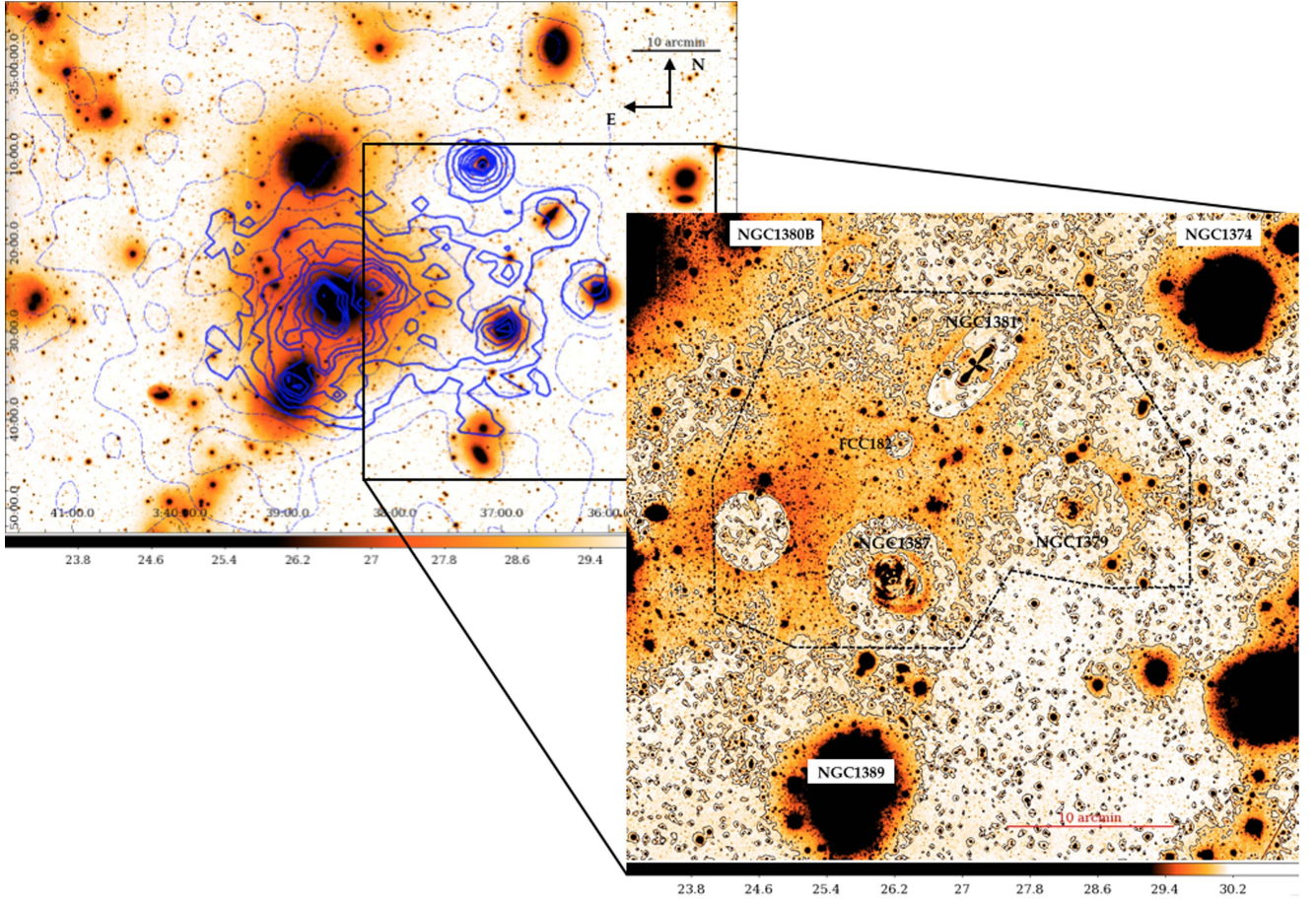
Figure 1. Left panel—central regions ( 2 \times 1 degrees 2 ) of the Fornax cluster in the r -band surface brightness levels. The blue GCs are derived by D’Abrusco et al. (2016; solid lines) and by Cantiello et al. (2017; dashed lines). Right panel—enlarged regions on the west side ( 40.9 \times 42.7 arcmin \sim 237 \times 248 kpc), where the bright galaxies were modeled and subtracted. In this area, the diffuse ICL is the central over-density that fills the intracluster space. The black contours are the surface brightness levels \mu_r = 29.8\text{--}30.02 mag arcsec -2 . The black dashed region marks the polygon aperture used to measure the integrated magnitudes of the ICL (see Section 3.1).
