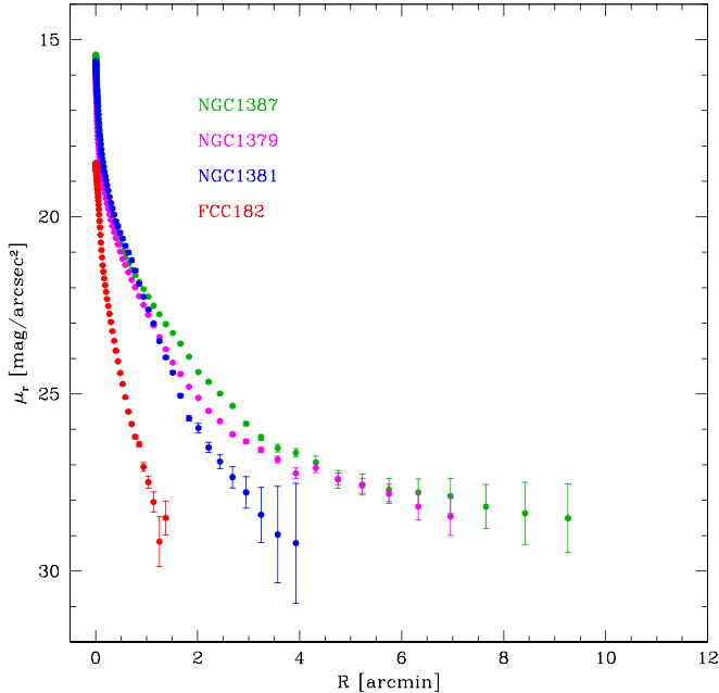
Figure 2. Azimuthally averaged surface brightness, in the r band, for the three brightest ETGs (NGC 1387, NGC 1379, and NGC 1381) and for the dwarf elliptical FCC 182 close to the ICL region.
