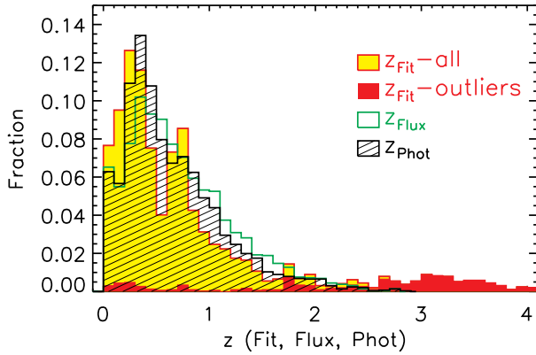
Figure 7. Redshift distribution in the SIMES field for 24 \mu\text{m} detected sources ( F_{24} > 0.3 \text{ mJy} ) resulting from SED fitting (red and yellow), optical flux analysis (green) and combined technique (black filled). The red filled distribution represents the identified outliers before the correction.
