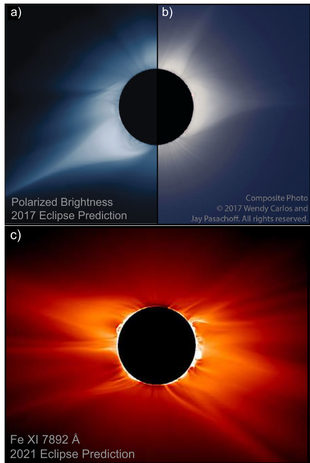
Figure 12 Two examples of forward modeling from the PSI eclipse predictions. Top panels: a merged image comparing the polarized brightness prediction for the 21 August 2017 total solar eclipse ( a ) to a processed eclipse photo ( b , images adapted from Mikić et al., 2018, and used with permission). Panel c shows radially filtered, sharpened radiances for the photoexcited Fe XI 789.2 nm emission line for the 14 December 2021 eclipse prediction ( predsci.com/eclipse2021 , see Boe et al., 2022, for details on the method).
