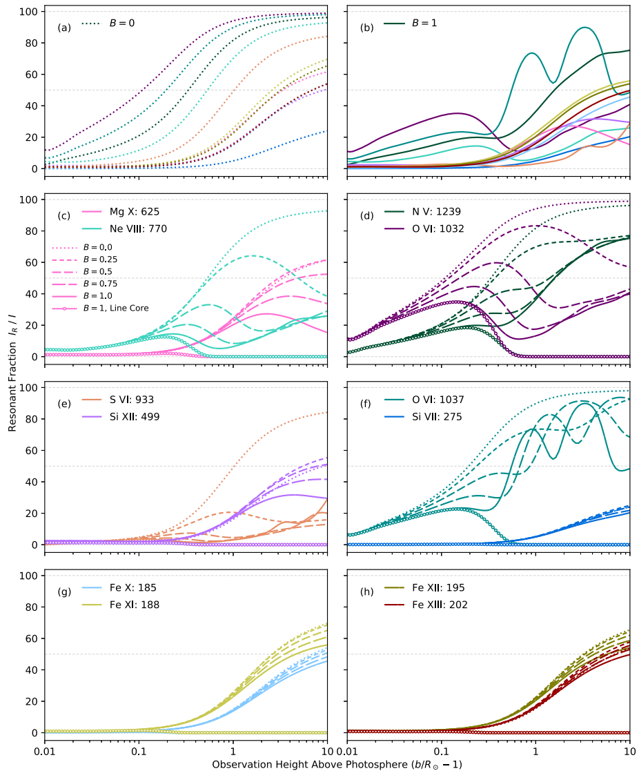
Figure 4 The proportion of the total emissivity contributed by resonant scattering as a function of height, for various fractions [B] of the model value of the solar-wind speed, as reported in Gilly and Cranmer (2020). B is a scalar factor applied to the radial-wind-speed profile, with B = 0 indicating no wind and B = 1 indicating wind at nominal modeled values. Ion-line wavelengths are given in units of angstroms. (Figure 17 of Gilly and Cranmer, 2020, used with permission).
