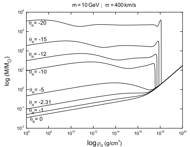
FIG. 3: Mass M of the equilibrium configurations in function of central density \rho_0 , at different values of \theta_R . A phase transition from non-quantum to fully degenerate configurations at densities around 10^{18} \text{ g cm}^{-3} is clearly visible.
