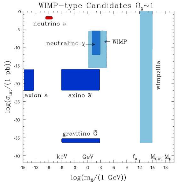
FIG. 2: A partial review of different DM candidates (particles only; adapted from [4]).
