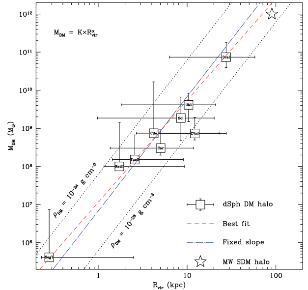
FIG. 8: Scaling relation for nine dSph DM halo parameters obtained from the Jeans analysis performed with the CLUMPY software ( open squares ) and MW parameters for the theoretical DM halo constructed with SMPs ( open star ). The errors at 68% confidence level are associated to the measurements of halo masses and virial radii. For comparison, the relation M_{\text{DM}} \propto R_{\text{vir}}^3 ( dashed line ) – corresponding to the average density of \sim 1.26 \cdot 10^{-25} \text{ g cm}^{-3} – is reported, along with the same relation scaled at 10^{-24} and 10^{-26} \text{ g cm}^{-3} ( dotted lines ).
