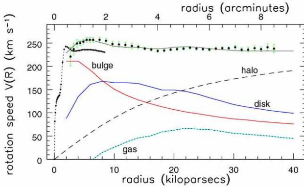
FIG. 1: Different components in our Galaxy (spiral) and contribution to the rotation curve (figure by K. Begeman & Y. Sofue adapted from [61]).
