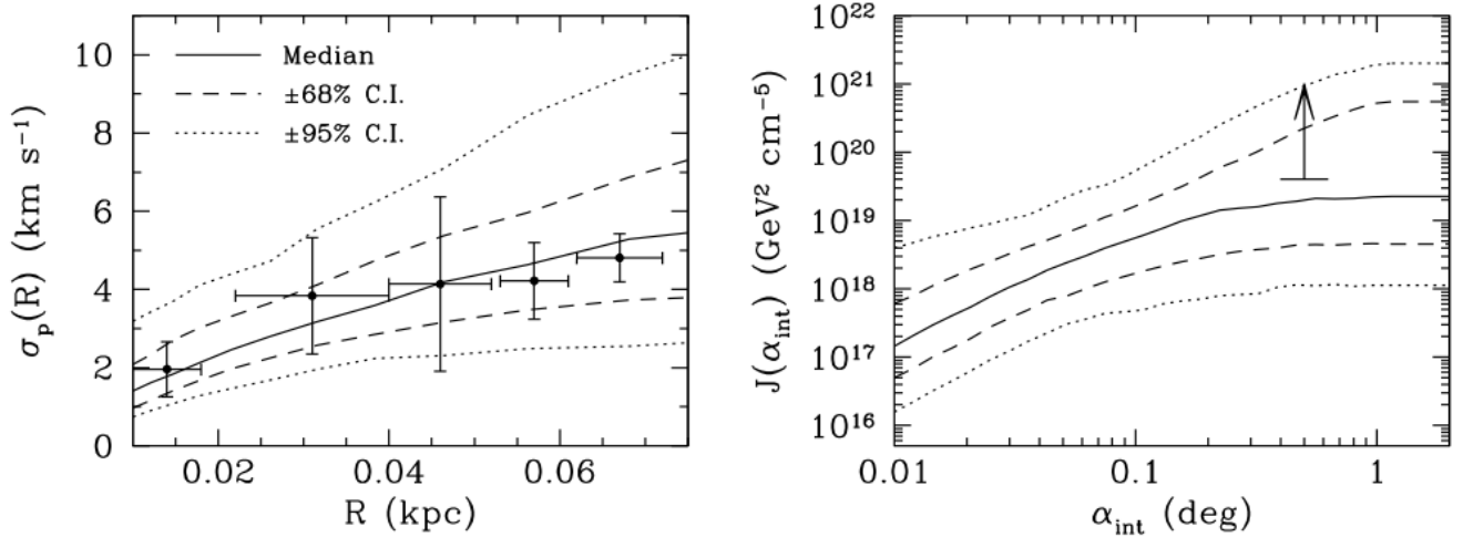
FIG. 7: Left panel: Ret II stellar velocity dispersion as a function of the projected radius from the dSph center obtained from the MCMC Jeans analysis. The median profile ( solid line ) is shown together with the corresponding confidence intervals at 68% ( dashed lines ) and 95% confidence level ( dotted lines ). For comparison, the binned measurements from [96] ( dots ) are overplotted together with their 1\sigma errors computed over the identified member stars. Right panel: Ret II astrophysical factor for DM annihilation as a function of the instrumental integration angle. The median profile ( solid line ) is shown together with the corresponding confidence intervals at 68% ( dashed lines ) and 95% confidence level ( dotted lines ). The lower limit on J(\alpha_{\text{int}}) derived by [73] is reported as a visual confirmation of the goodness of the MCMC calculations.
