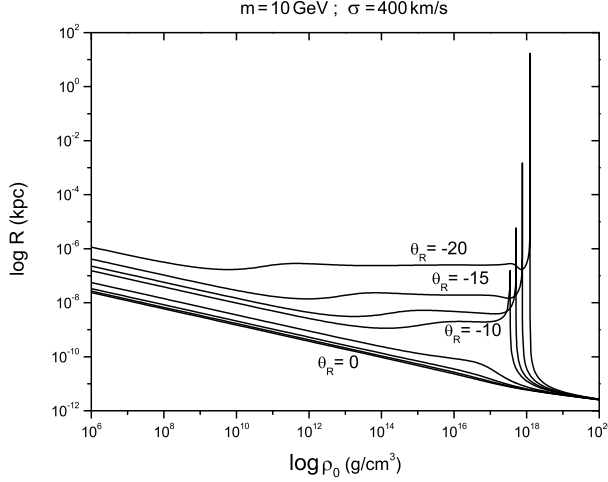
FIG. 4: Radius R of the equilibrium configurations in function of central density \rho_0 , at different values of \theta_R . A phase transition from non-quantum to fully degenerate configurations at densities around 10^{18} \text{ g cm}^{-3} is clearly visible.
