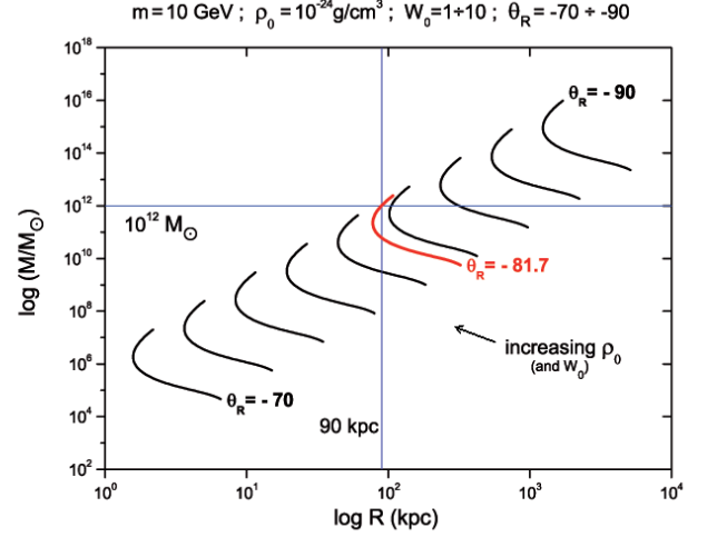
FIG. 5: Identification of the value of \theta_R compatible with the required values of mass and radius for spiral-galaxy halos. The position of a MW-sized halo (blue axes) is highlighted, along with the relevant value of \theta_R (red curve).
