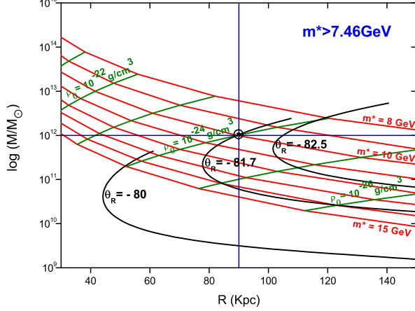
FIG. 6: Solutions for MW-sized DM halos obtained through scaling laws between halo physical parameters and conglomerate masses. The relations between halo mass and size for different conglomerate masses (red curves), DM central densities (green curves) and concentration parameters (black curves) are plotted. The position of the MW-sized halo for m^* = 10 GeV (open circle with dot) is also marked.
