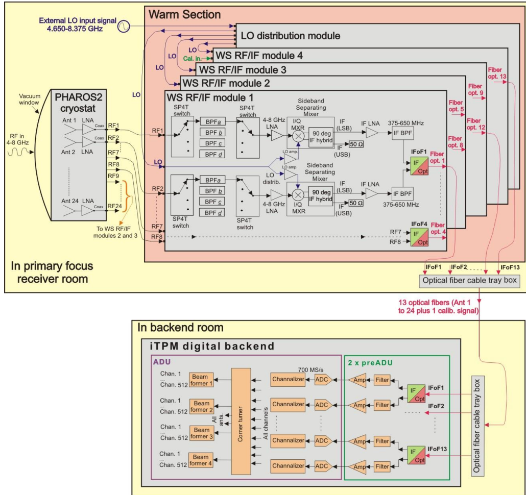
FIG. 4 – Schematic diagram of PHAROS2.
