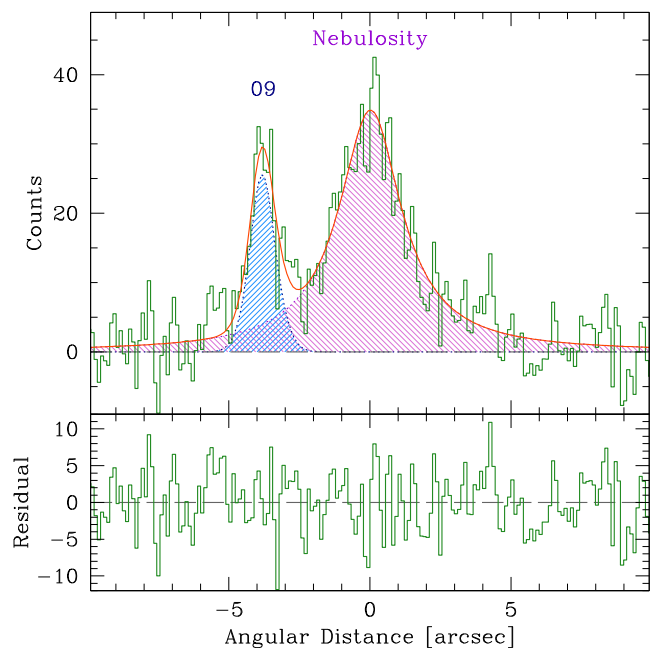
Figure 3. Example of our deblending procedure on a 3 pixel slice of the 2D long-slit spectrum centred at \lambda = 5500 Å. Top panel: spatial profile of the two spectra (green line). The contributions of PKS 2155–304_09 and of the PKS 2155–304's nebulousity were deblended performing a simultaneous fit with a Gaussian and a Lorentzian function, respectively (blue and purple shaded areas). The result of the fit is also shown (orange line). Bottom panel: residual spectrum.
