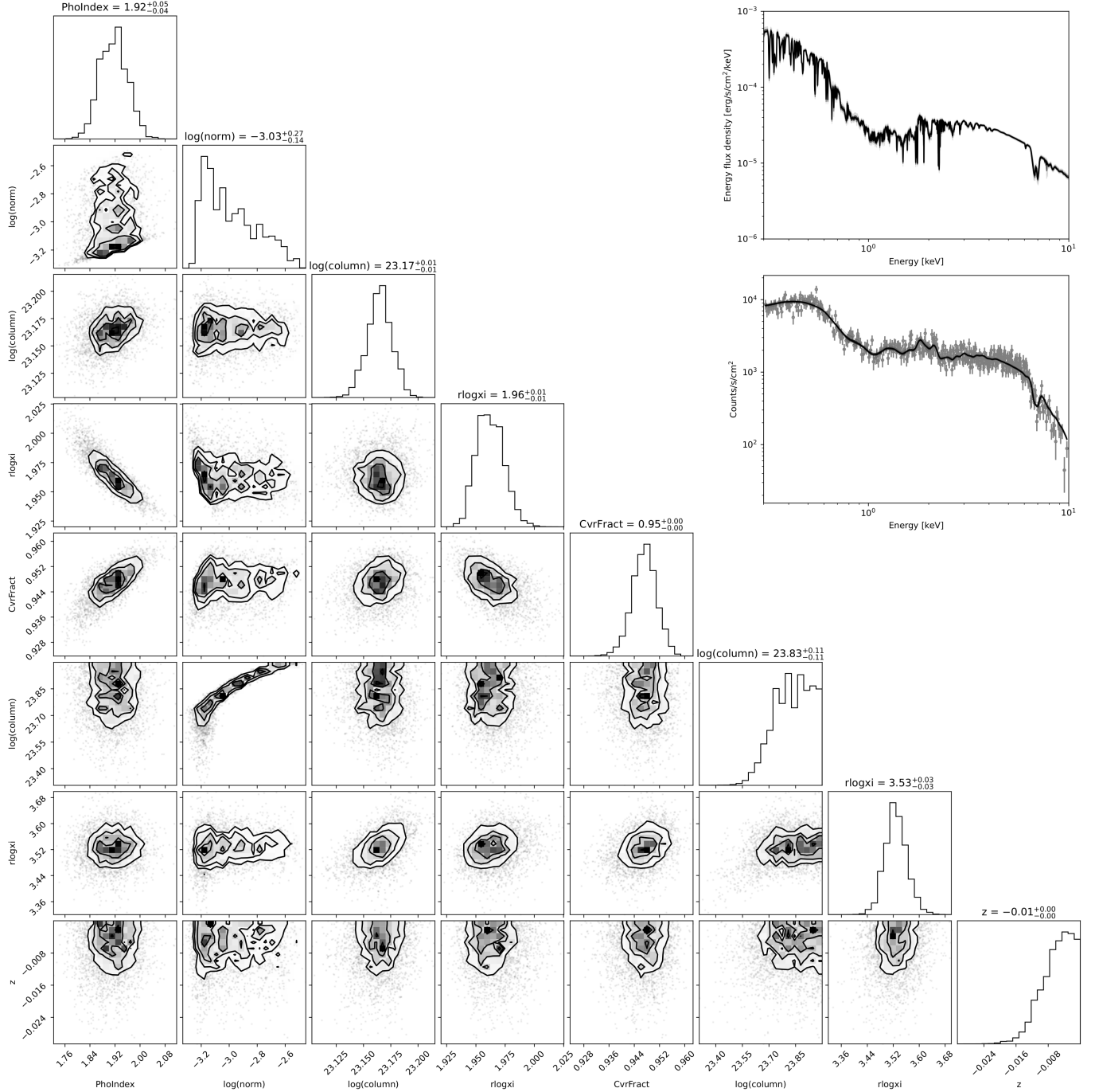
Fig. A.1. Bayesian analysis results for the parameters of the model [(\text{partcov} \times \text{xstar500}) * (\text{xstar5000} * \text{pow})] given the 2009 data. The corner plot reports the 1D (histograms) and 2D (credible contours) posterior probability distributions for the model parameters. The top right panels report the posterior probability distributions of the theoretical model (top) and of the model convolved with the instrumental response, with the binned EPIC-pn data overplotted (bottom).
