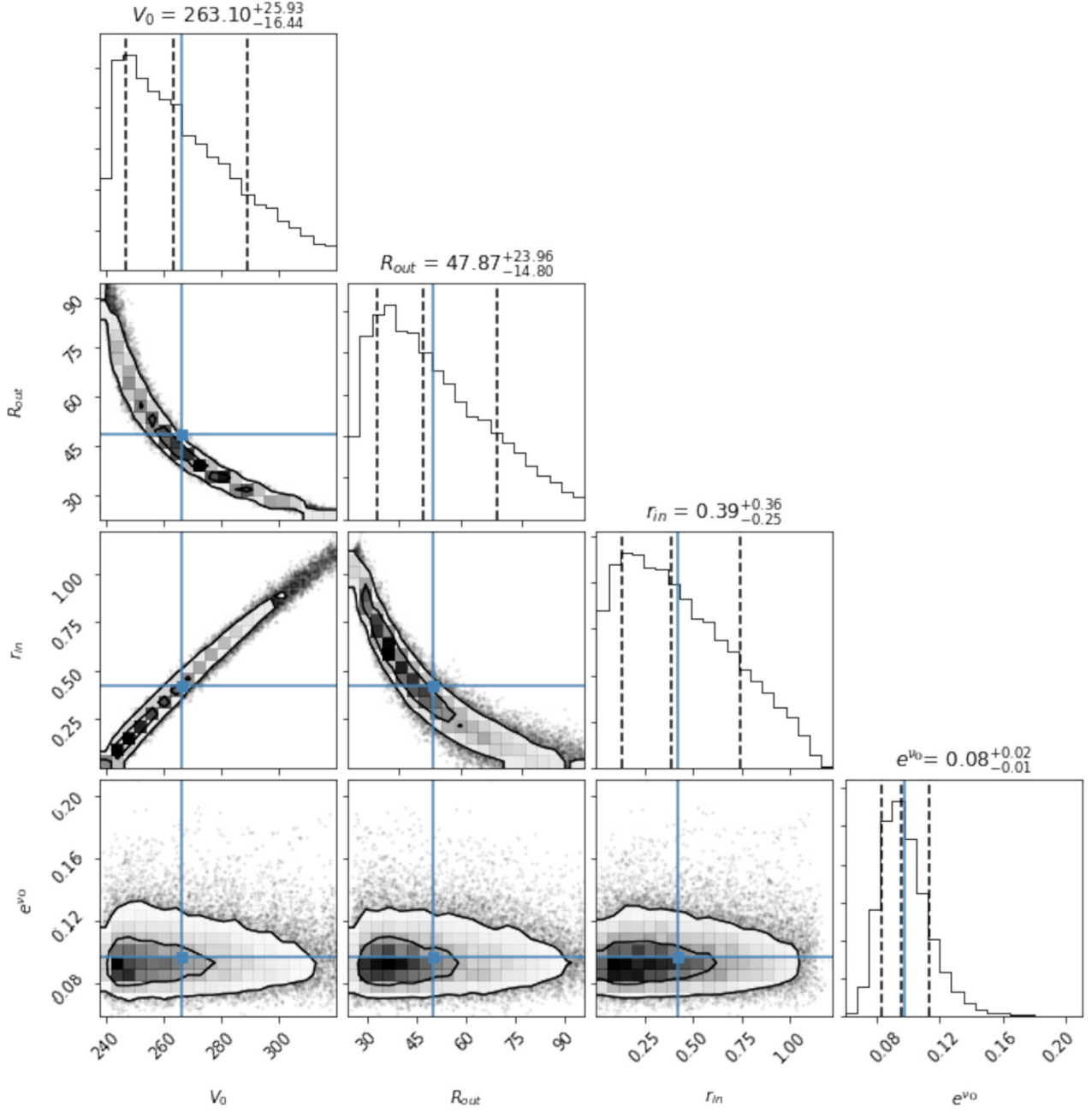
Figure C2. BG parameters corner plot. Same as in Figure C1.
