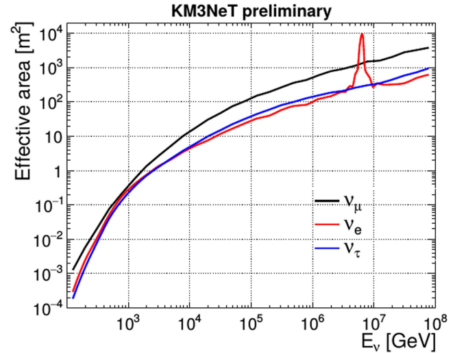
Figure 3. This plot is taken from Andrián-Martínez et al. (2016), it shows the effective areas of ARCA (two blocks) at trigger level for \nu_\mu , \nu_e and \nu_\tau , as a function of neutrino energy E_\nu . The effective area is defined relative to an isotropic neutrino flux incident on the Earth, is averaged over both \nu and \bar{\nu} , and includes both NC and CC interactions. The peak at 6.3 PeV is due to the Glashow resonance of \bar{\nu}_e .
