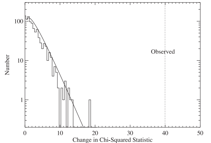
Figure 4. Results of Monte Carlo simulations for testing line significance for continuum model II (Section 5). We simulated 1000 fake NuSTAR spectra for the continuum-only model (bbodyrad + cut-offpl), and attempted to fit them with a continuum+line model with N_H fixed at the value obtained with a joint Swift /XRT fit. The solid histogram shows \Delta\chi^2 values obtained in the simulations, and the smooth curve is a \chi^2 distribution with 3 degrees of freedom. The \Delta\chi^2 attained in actual data (dashed vertical line) is significantly higher than values attained in simulations. This \Delta\chi^2 value differs that in Table 3 due to the simplifying assumptions made in these simulations (Section 5).
