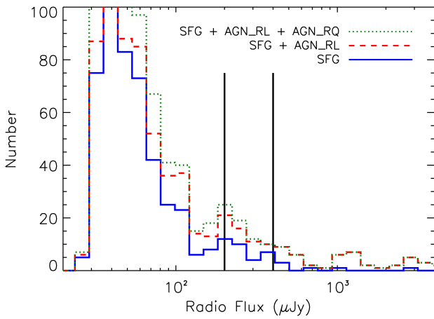
Fig. 1. Stacked histogram of the radio flux density distributions of the sources in Bonzini et al. (2013) . The solid blue curve refers to SFGs, the red dashed curve adds to it the RL AGNs, the green dotted curve adds to them the secure (QF = 3) RQ AGNs. The two black vertical lines delimit the flux range of the sample we targeted (200–400 \mu\text{Jy} ).
