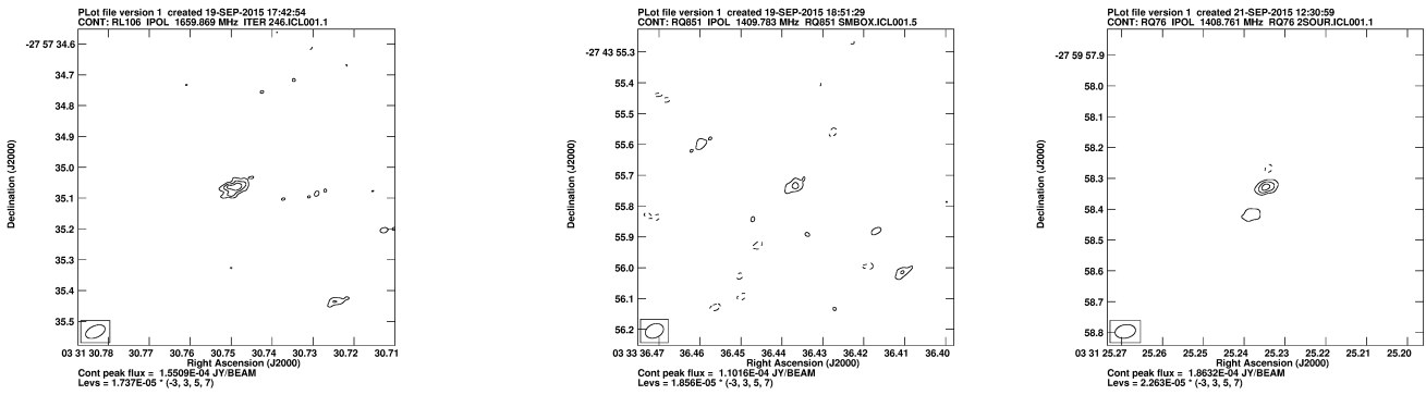
Fig. 2. Images of the VLBI-detected sources: RL 106 ( Left ), RQ 851 ( Centre ), and RQ 76 ( Right ). All the isophotes are drawn at -3 , 3 , 5 and 7 times the image 1\sigma noise ( 17.4 , 18.6 and 22.6\mu\text{Jy} , respectively). All images are \sim 1 \times 1 \text{ arcsec}^2 wide.
