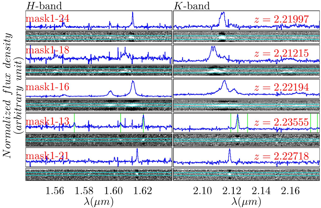
Figure 2. Example 2D and extracted 1D spectra showing some emission lines. Cyan lines show the 1D extraction window. The position of H\beta , [O\text{ III}]\lambda 4959 , [O\text{ III}]\lambda 5007 , [N\text{ II}]\lambda 6549 , H\alpha , [N\text{ II}]\lambda 6583 , [S\text{ II}]\lambda 6717 , and [S\text{ II}]\lambda 6731 emission lines is shown with vertical green lines for one of the galaxies. The top two spectra show two merger cases, the third one is a broad-line AGN, and the last two spectra show normal star-forming galaxies in the protocluster.
