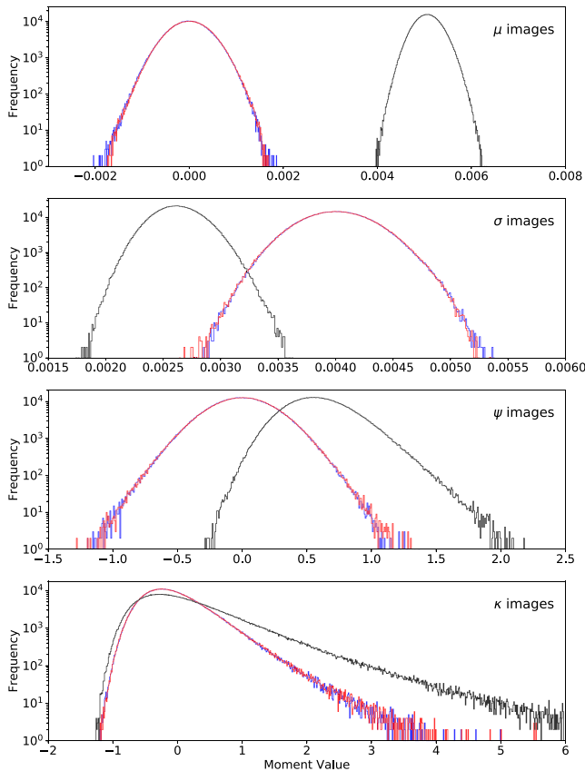
Figure 6. The distributions of noise in the central region of 1024^2 pixels in the moment images, as derived from a simulated data cube that contains no sources. The distributions are shown for Q (blue), U (red), and P (black). The noise distributions of the moment images for the mean \mu (top panel), standard deviation \sigma (2nd panel), skewness \psi (3rd panel), and excess kurtosis \kappa (bottom panel), are all shown. Note that the y-axis is shown as a log-scale in order to accentuate deviations from a normal distribution.
