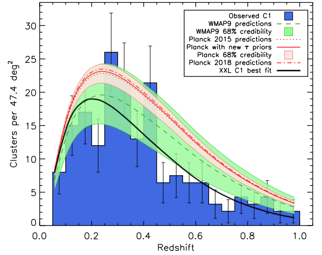
Fig. 1. The histogram shows the observed redshift distribution of the 178 XXL C1 clusters used in the present study. Errors bars account for shot noise and sample variance following Valageas et al. (2011); the cluster deficit at z \sim 0.5 is present in both the XXL-N and XXL-S fields. Overlaid, the modelling obtained for different cosmologies assuming the cluster scaling relations of Table 1. The green line shows the prediction from the mean WMAP9 cosmology. The red dotted line corresponds to the Planck 2015 parameters (TT+lowTEB+lensing) of Planck Collaboration et al. (2016a). The red full line shows the prediction from our reanalysis of the Planck 2015 data adopting the updated estimate of the optical depth to reionisation \tau presented in Planck Collaboration et al. (2016e), which we describe in Appendix B. For comparison we also show the prediction of the recent Planck 2018 analysis Planck Collaboration et al. (2018) which includes the final polarisation analysis (dot-dashed line). The shaded areas around model predictions correspond to uncertainties on the corresponding cosmological parameters, but do not include any error on scaling relations. Finally, the black thick line shows our best-fit \Lambda CDM model to the XXL clusters of subsection 3.2, which provide a very good fit to the data.
