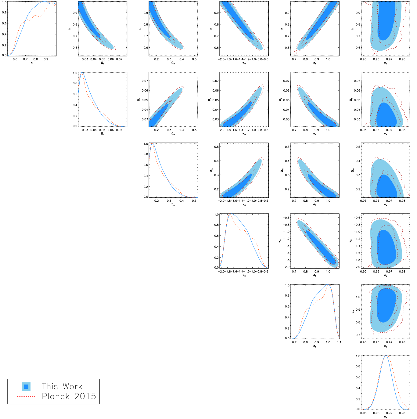
Fig. B.2. Comparison of the cosmological analysis of the Planck CMB products used in this paper with the original constraints of Planck Collaboration et al. (2016a) in a flat w CDM universe ( 1\sigma and 2\sigma contours).
