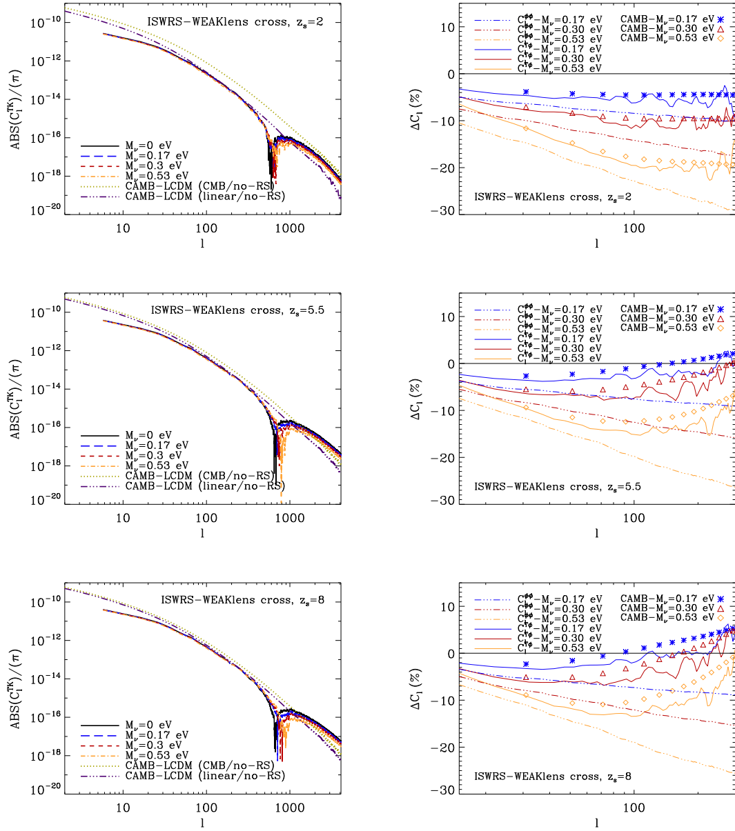
Figure 9: Left: absolute values of the WL/ISW-RS angular cross spectra for sources placed at redshifts z = 2 (upper panel), z = 5.5 (middle panel), and z = 8 (lower panel), respectively. The solid black, long-dashed blue, dashed red, and dot-dashed orange lines represent the simulated signals for M_\nu = 0, 0.17, 0.3, 0.53 eV, respectively. The \Lambda CDM linear expectations from CAMB are represented by the tri-dotted violet line. The light-green dotted line is the linear ISW-RS/CMB-lensing cross spectrum from CAMB, here shown for comparison. Right: percent residuals wrt the massless case for l < 300 . Tri-dot-dashed blue, red, and orange lines correspond to the simulated signals of the auto WL power spectra for M_\nu = 0, 0.17, 0.3, 0.53 eV, respectively. Solid blue, red, and orange lines are the residuals of the simulated ISW-RS/WL cross spectra. The corresponding semi-analytical linear CAMB predictions are represented by symbols, as described in the legend.
