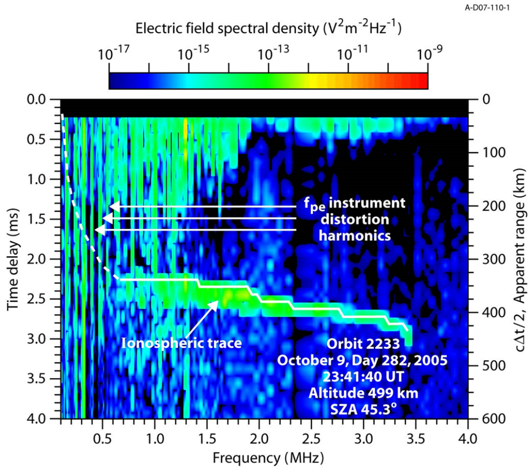
Figure 3: A sample ionogram (from Morgan et al., 2008).
