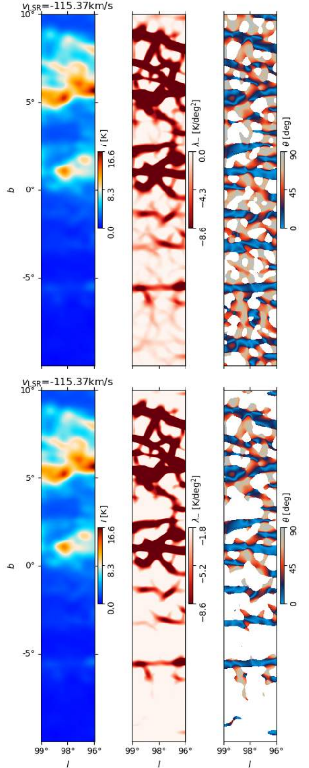
Fig. A.11: Example of the filamentary structures identified using the Hessian method with curvature thresholds \lambda_- < 0 (top) and \lambda_- < -1.8 \text{ K deg}^{-2} (bottom). The three maps represent: Left : HI intensity after the smoothing by a Gaussian kernel with the size of the derivative kernel. Center : Second eigenvalue of the Hessian matrix, \lambda_- , calculated using Eq. 2. Left : Filament orientations, \theta , calculated using Eq. 3. The radial velocity corresponds to a kinematic distance d = 12.7 \text{ kpc} and Galactocentric radius R_{\text{gal}} = 16.1 \text{ kpc} , as derived using the assumptions in App. B
