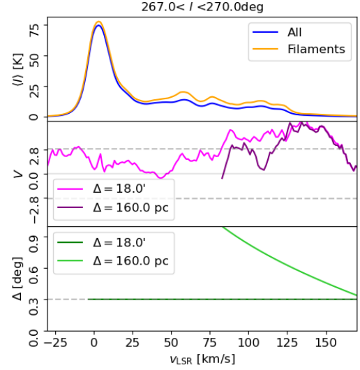
Fig. 5. Mean intensity ( \langle I \rangle , top), projected Rayleigh statistic ( V , middle), and derivative kernel size ( \Delta , bottom) for 3^\circ \times 20^\circ \times 1.29 \text{ km s}^{-1} toward the indicated positions. The two lines in the middle panel indicate the results obtained with a derivative kernel with a fixed angular size and a kernel with a fixed physical size, as indicated on the legend. The kernel with a fixed physical size is exclusively used in the radial velocity range corresponding to kinematic distances where the angular size of the kernel is below 1^\circ .
