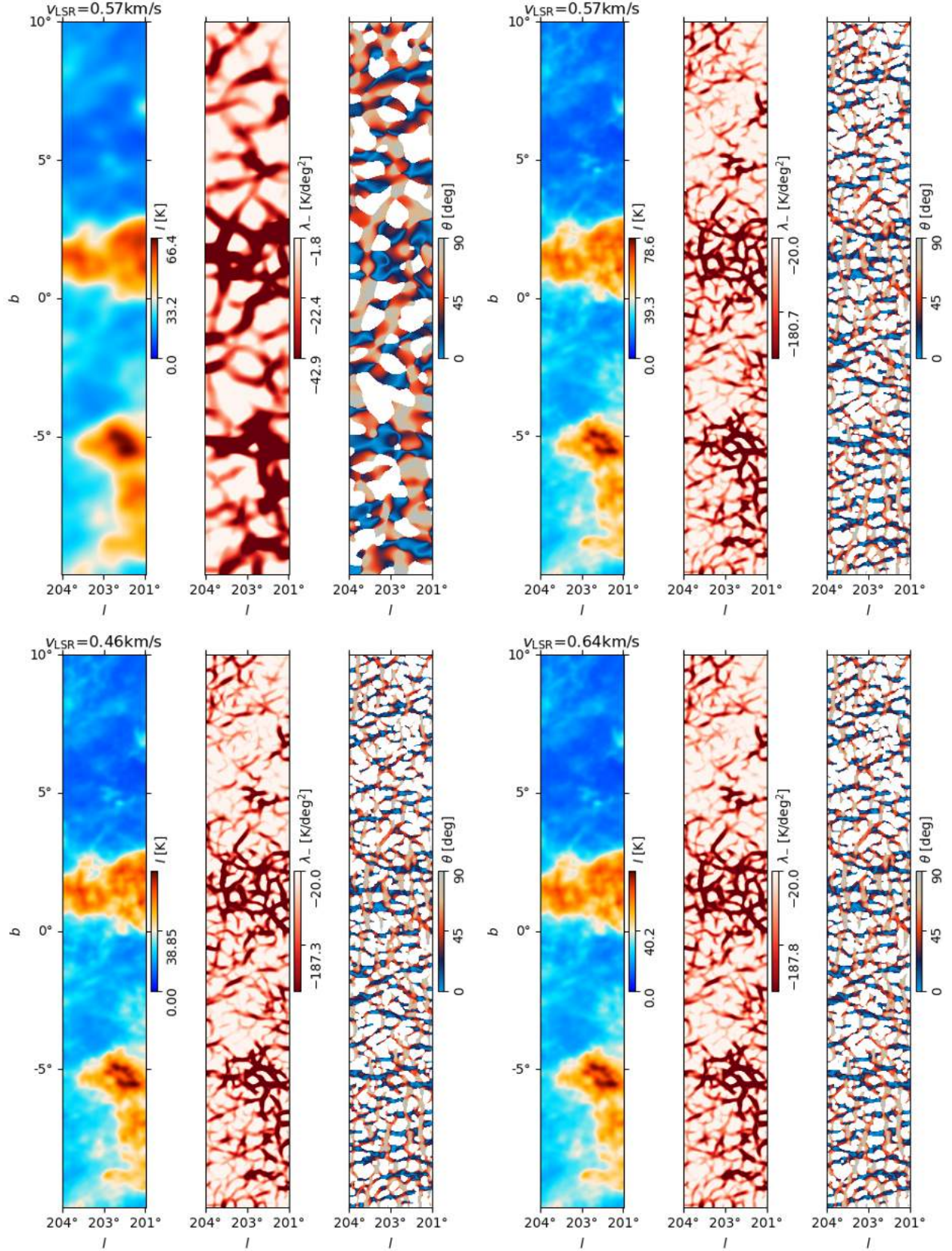
Fig. C.1: Hessian matrix analysis applied to the HI4PI and the GALFA-HI observations. Top . Results obtained on a 3^\circ \times 20^\circ \times 1.29 \text{ km s}^{-1} tile in the HI4PI and the GALFA-HI observations, shown in the left and right panels, respectively. Bottom . Results obtained on two 3^\circ \times 20^\circ \times 0.184 \text{ km s}^{-1} tiles in the GALFA-HI observations. In each of the panels, the left-hand side map shows the HI emission convolved with a 2D Gaussian with the same diameter of the derivative kernel. The map in the center shows the second eigenvalues of the Hessian matrix, \lambda_2 , which highlights the filamentary structure. The right-hand side map shows the orientation angle of the filamentary structure.
