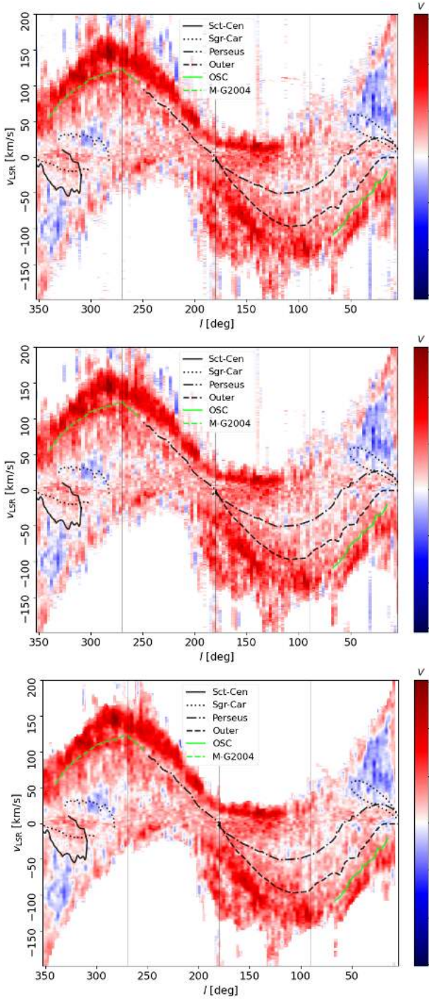
Fig. A.10: Same as Fig. A.7, but for 3^\circ \times 20^\circ \times 1.29 \text{ km s}^{-1} tiles and intensity thresholds of 3\sigma (top), 5\sigma (middle), and 9\sigma (bottom).
