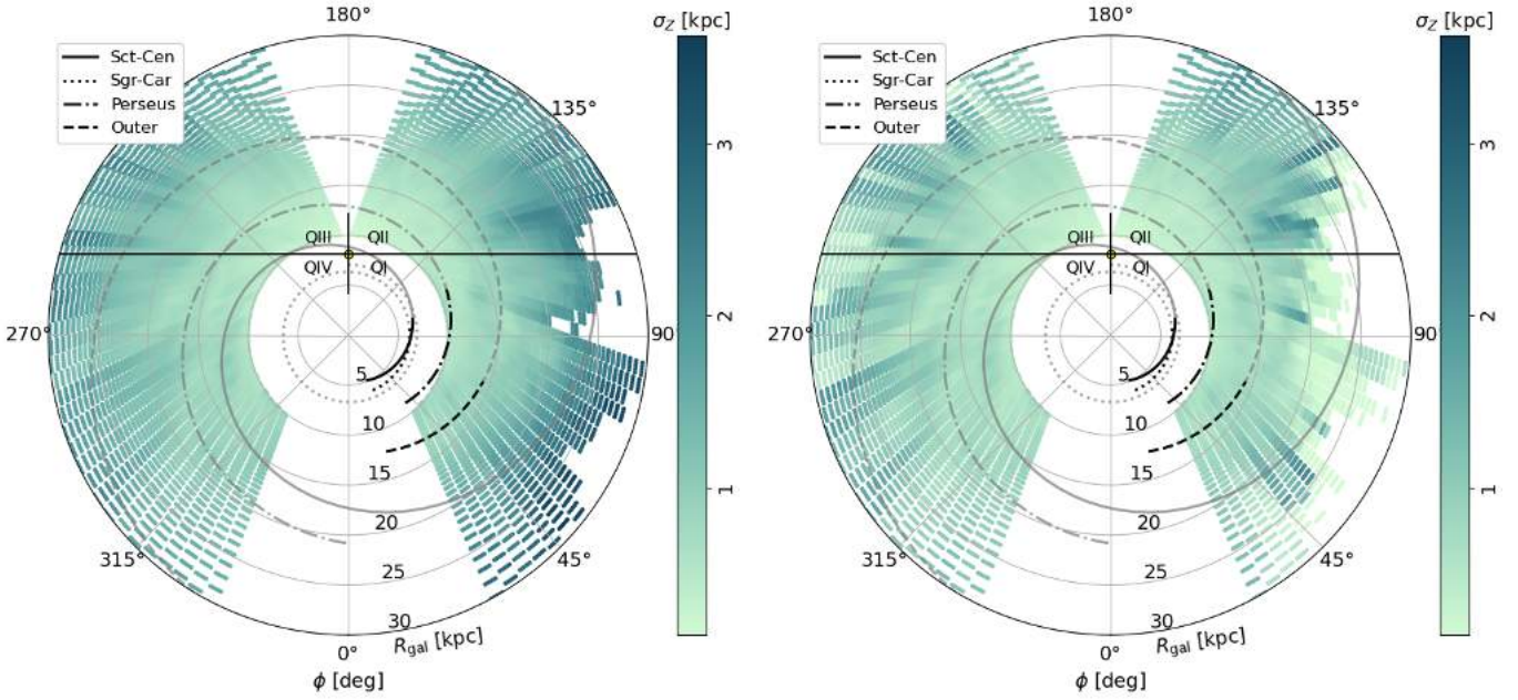
Fig. 10. Face-on view of the dispersion around the midplane height ( \sigma_z ) reconstructed from all the emission in the range |b| < 10^\circ (left) and the emission in filamentary structures (right).
