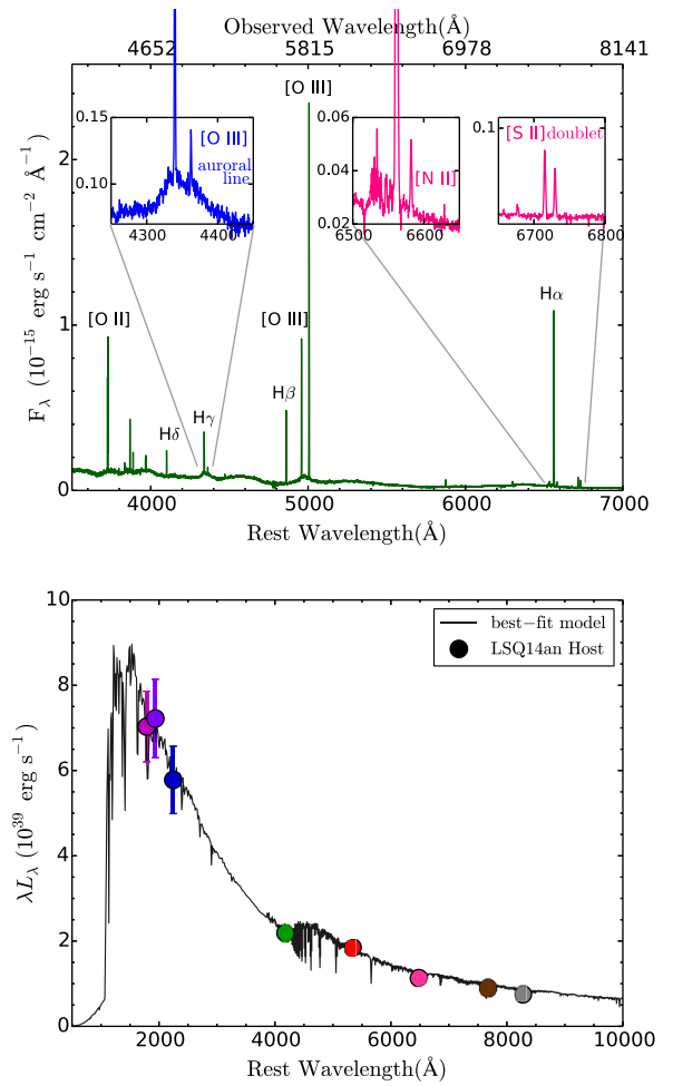
Figure 2. Top: spectrum of the host of LSQ14an taken by VLT+X-Shooter on 2014 June 21. The spectrum in the merged data from the UVB, VIS and NIR arms, corrected to rest frame. Host lines are labelled in the spectrum. Bottom: the best-fitting SED of the host of LSQ14an from MAGPHYS (da Cunha, Charlot & Elbaz 2008) shown as black line. The coloured circles show photometry of LSQ14an host in the order of the Swift uvw2 , uvm2 , uvw1 and Pan-STARRS1 grizy filters.
