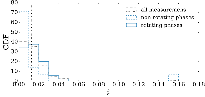
Fig. 9. J0324+3410: The distribution of the de-biased polarisation fraction \hat{p} . The dot-dashed vertical line marks the median of the distribution. The blue dashed line shows the distribution of \hat{p} during the non-rotating phases and the solid one that during the rotating phases. The black dotted line corresponds to all the measurements.
