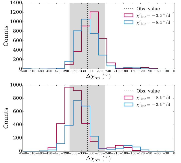
Fig. 7. J1505+0326: The distribution of rotation angles at the most likely intrinsic rotation rates based on the 1\sigma (upper panel) and the extreme-span-criterion (lower panel, case 3 of Section 5.1.3). The dashed line marks the observed value and the grey area the 1\sigma uncertainty.
