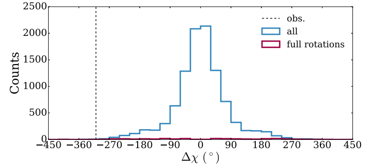
Fig. 5. J1505+0326: The distribution of \Delta\chi in the simulated EVPA curves where we assume the absence of intrinsic variability and the operation solely of noise. The dashed line is the observed rotation angle of 309.5^\circ .
