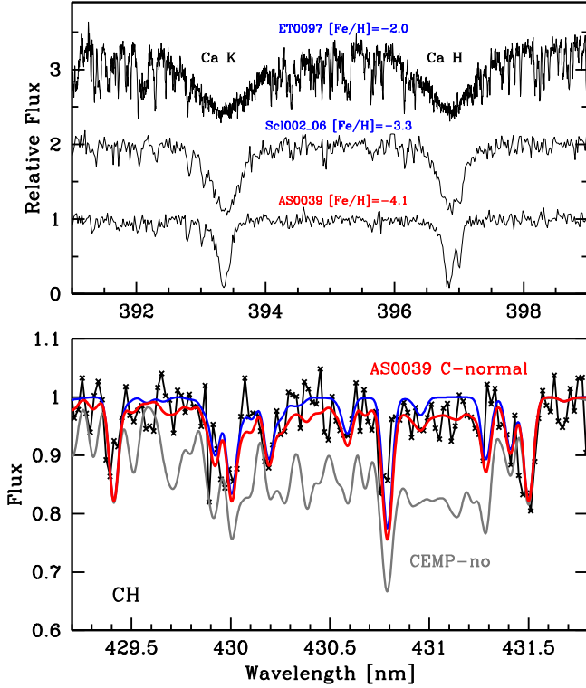
Figure 1. Spectrum of AS0039. Top panel: comparison to other metal-poor stars in Sculptor of similar temperature and gravity (Starkenburg et al. 2013; Skúladóttir et al. 2015b). Bottom panel: comparison of the CH G-band region of AS0039 to synthetic spectra: Red shows the best fit, blue is a synthetic spectrum with no CH lines, and gray represents a star born with the minimum amount of [C/Fe] = +0.7 to qualify as a CEMP-no star (accounting for mixing; Placco et al. 2014).
