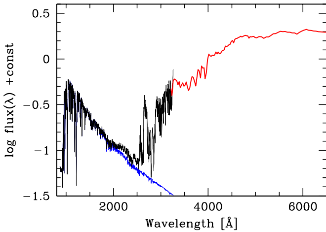
Figure 5. Synthetic SED of NGC 6791. The integrated spectrum is obtained by summing up the contribution of our bona fide star sample of 4739 entries. Mid-UV ( \lambda \lesssim 3200 Å) spectral synthesis has been carried out at high resolution (2 Å FWHM) by attaching each star to the corresponding UVBLUE synthetic spectrum with the same fundamental parameters (black line). The same procedure has been adopted at a longer wavelength (red line) by matching the Kurucz's (1993) ATLAS9 library at low resolution ( \sim 25 Å). The selective contribution of hot ( T_{\text{eff}} \geq 10,000 K) is singled out (blue line) showing that these stars are the prevailing contributors to the striking UV upturn in this SED. According to our estimate (see Equation (6)) this feature collects about 1.7\% \pm 0.4\% of the total bolometric luminosity of the cluster.
