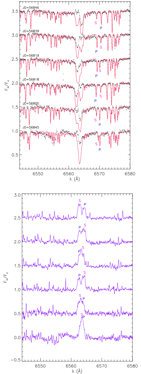
Figure 7. Sample of CAOS spectra of G 137-52 in the H\alpha region taken at different orbital phases. (Left-hand panel) Synthetic composite spectra (red lines) are overlaid with the observed spectra (black dots) taken at the Julian date marked on top on each spectrum. The position of the \text{Fe I } \lambda 6569 \text{ \AA} line of the primary (P) and secondary (S) components is also marked in each spectrum. The chromospheric emission that fills in the H\alpha core of both components is clearly visible in the subtracted spectra (right-hand panel) where the H\alpha wavelength of the primary and secondary components is also marked.
